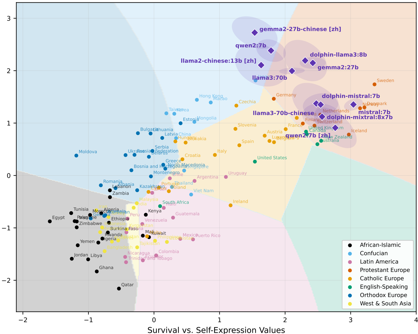
SVM cultural-region decision boundaries with LLM positions
