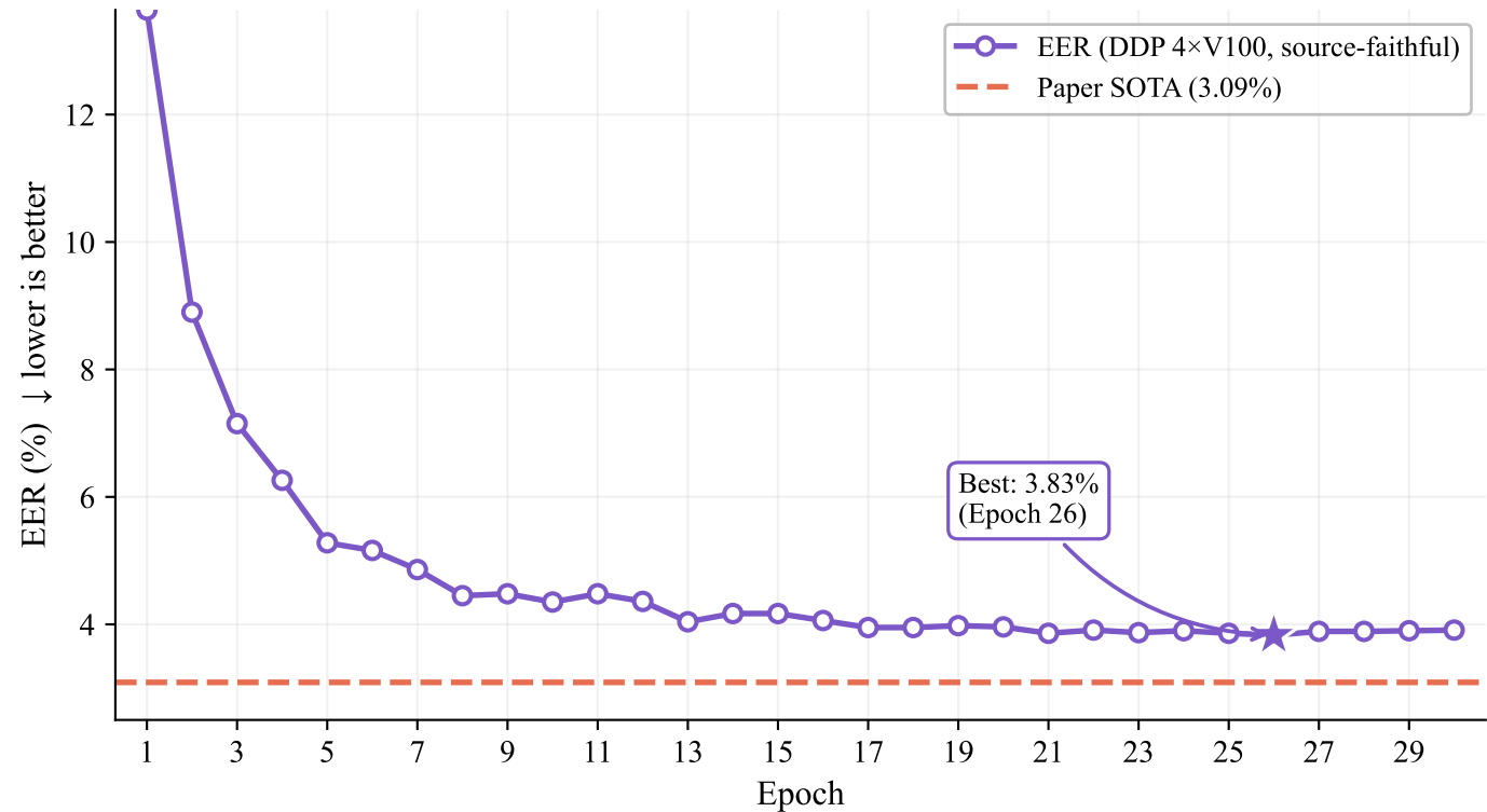
EER on VoxCeleb1 — CAARMA (DDP 4×V100, source-faithful)
