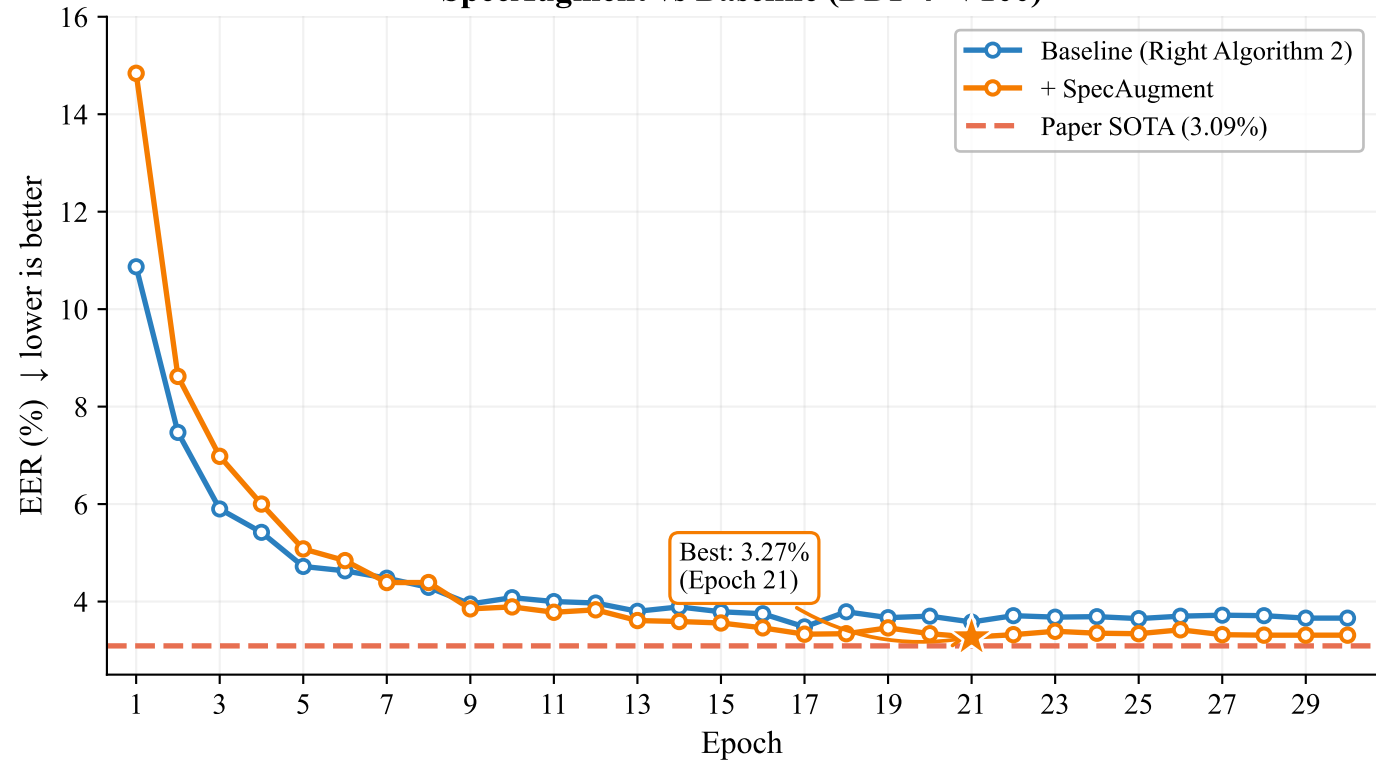
SpecAugment vs Baseline (DDP 4×V100)
