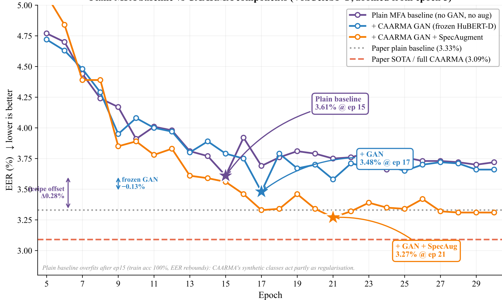
Plain MFA baseline vs CAARMA components (VoxCeleb1-O, zoomed from epoch 5)
