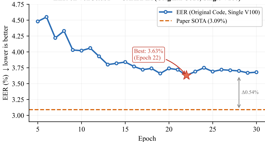
EER on VoxCeleb1 — CAARMA (Original Code, Single V100)
