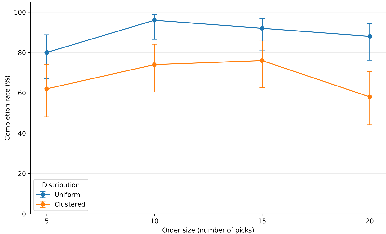
DQN Completion Rate by Order Size
