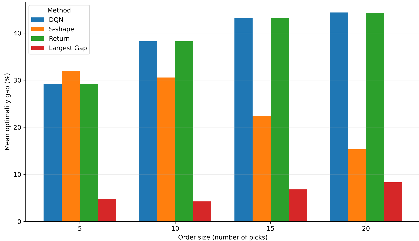
Mean Optimality Gap — Uniform Orders
