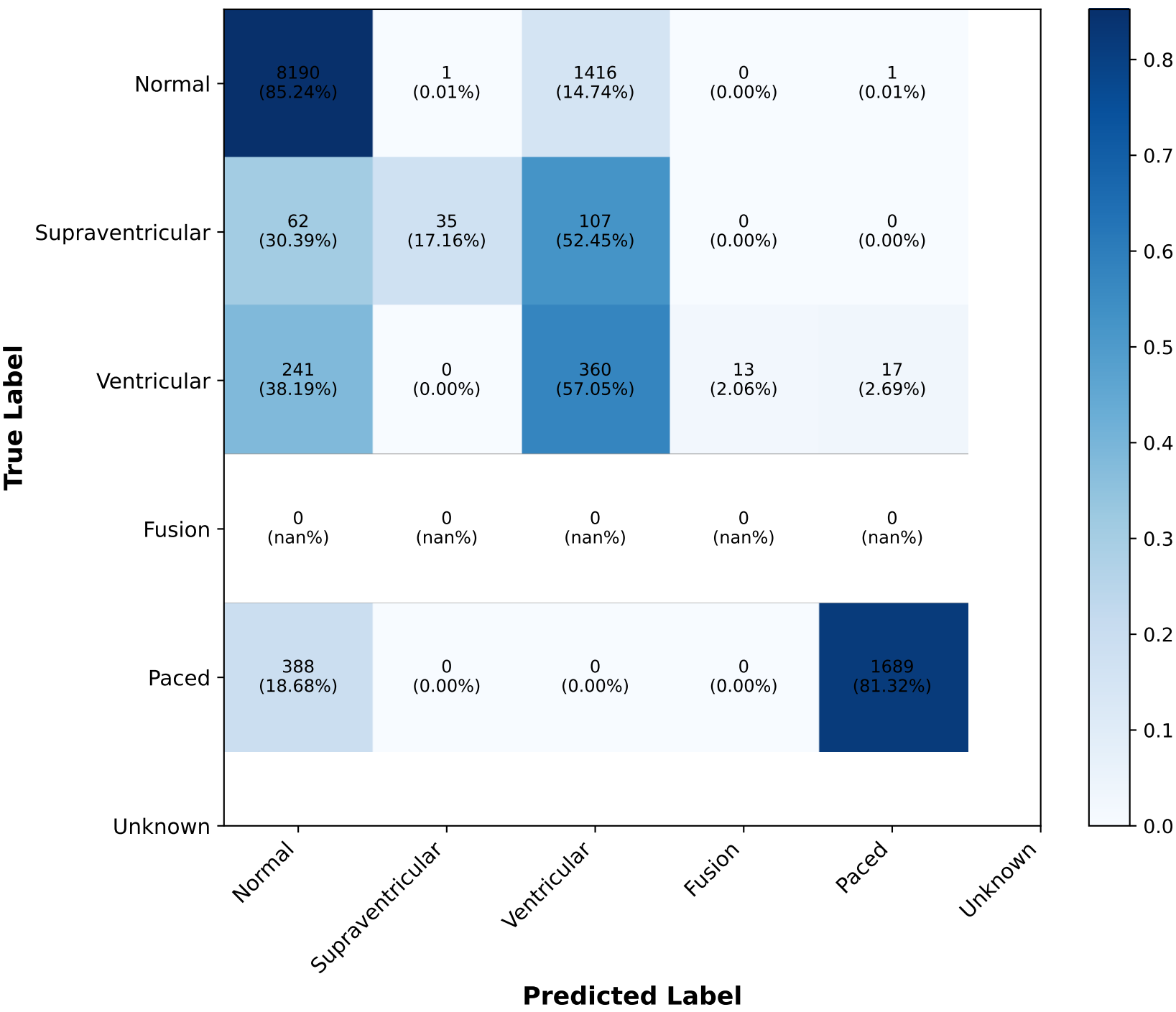
LSTM AUTOENCODER - Confusion Matrix
