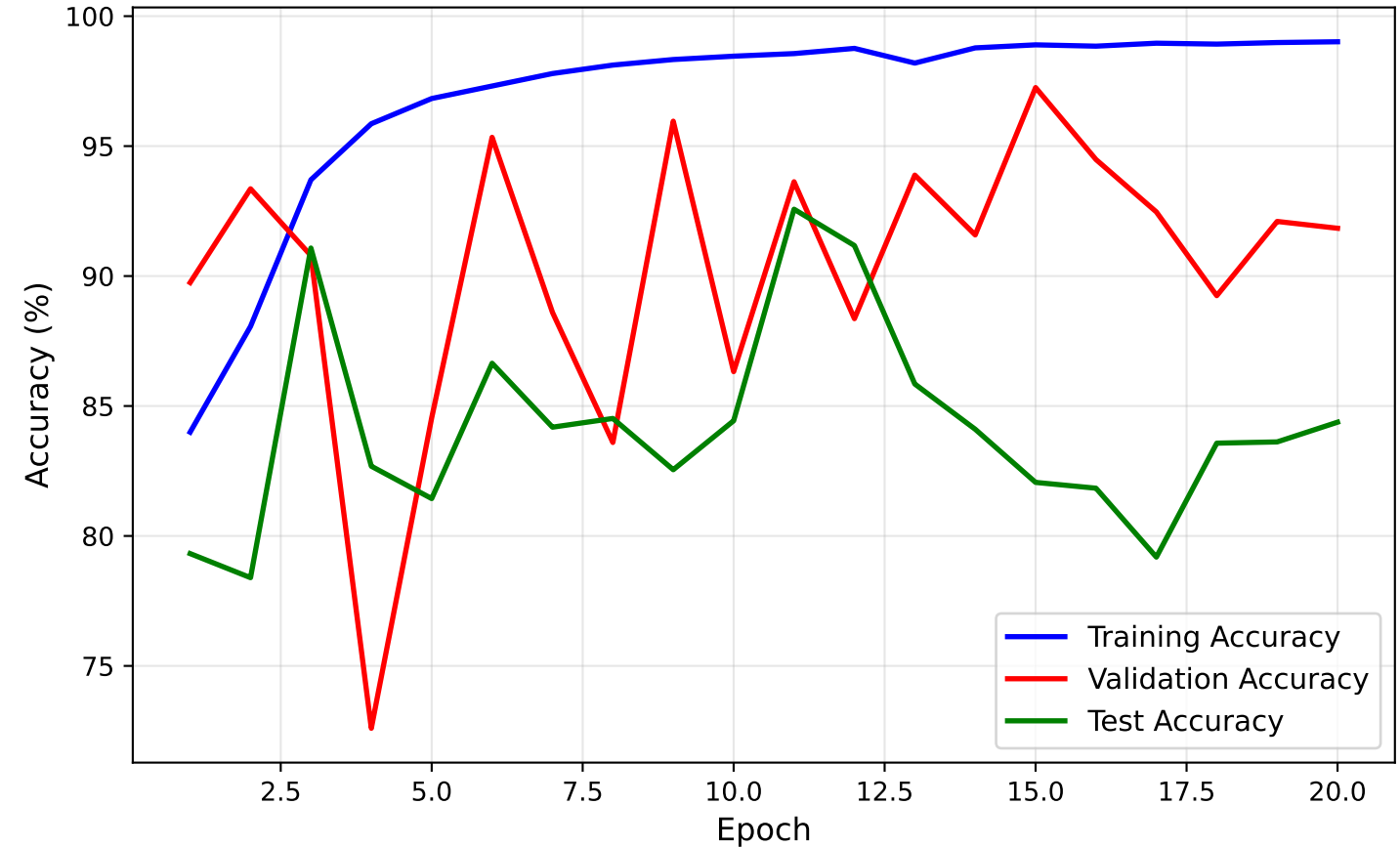
LSTM AUTOENCODER - Training/Val/Test Accuracy
