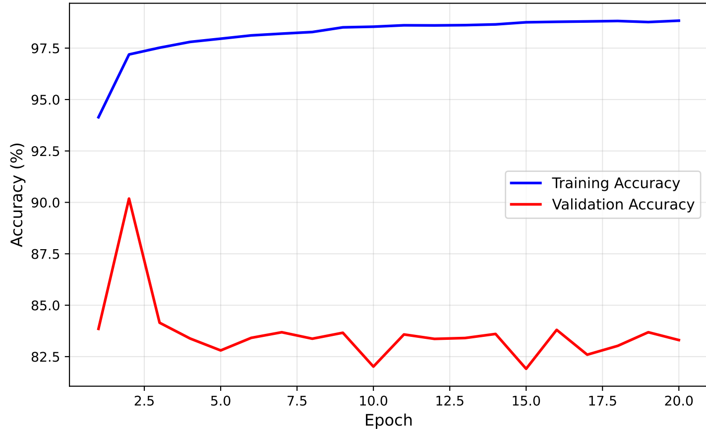
SIMPLE CNN - Training and Validation Accuracy
