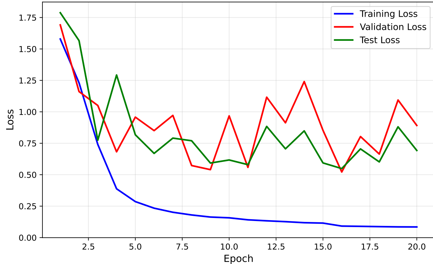
LSTM AUTOENCODER - Training/Val/Test Loss
