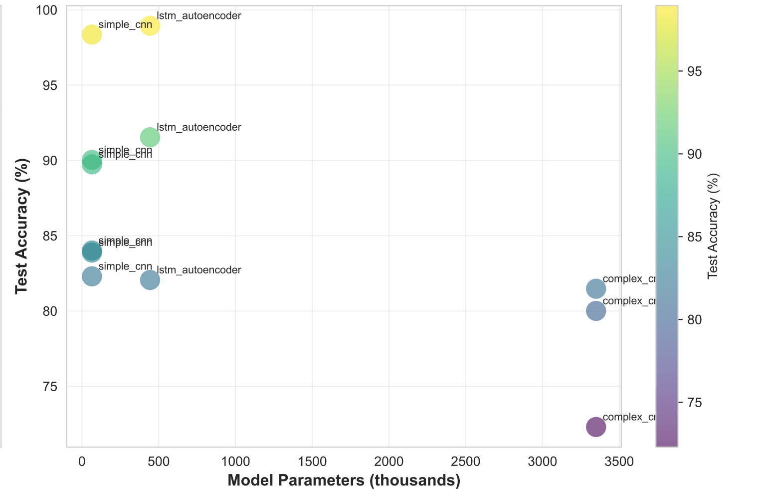
Model Size vs Performance
