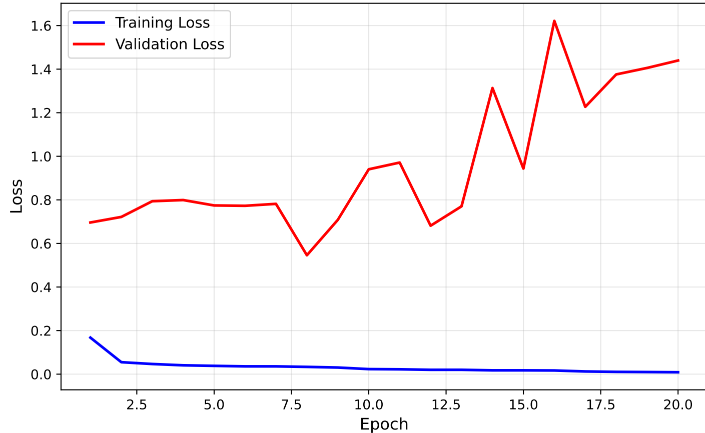
COMPLEX CNN - Training and Validation Loss
