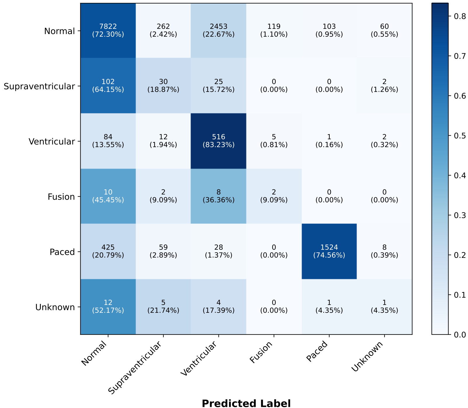
COMPLEX CNN - Confusion Matrix
