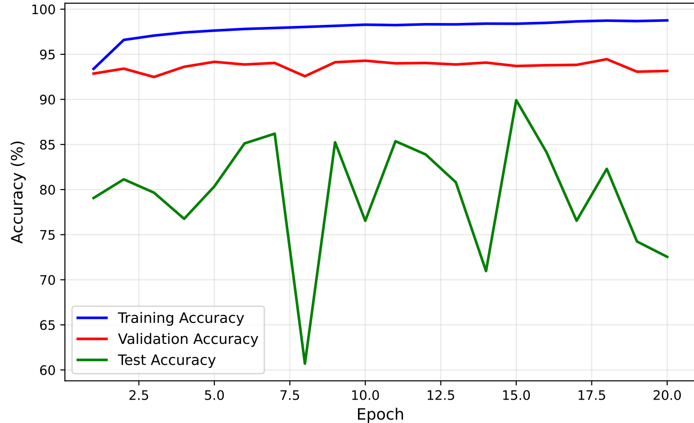
SIMPLE CNN - Training/Val/Test Accuracy
