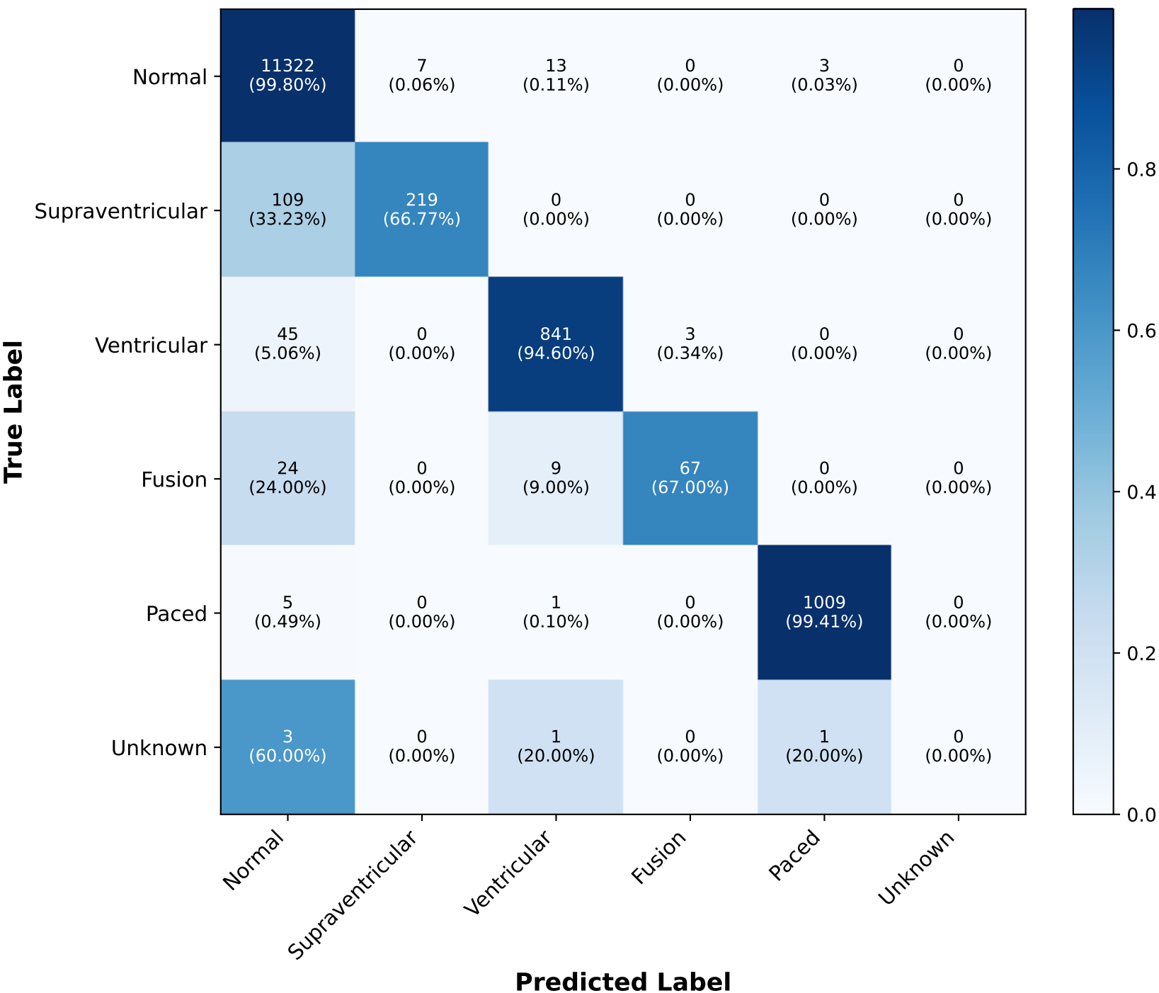
SIMPLE CNN - Confusion Matrix
