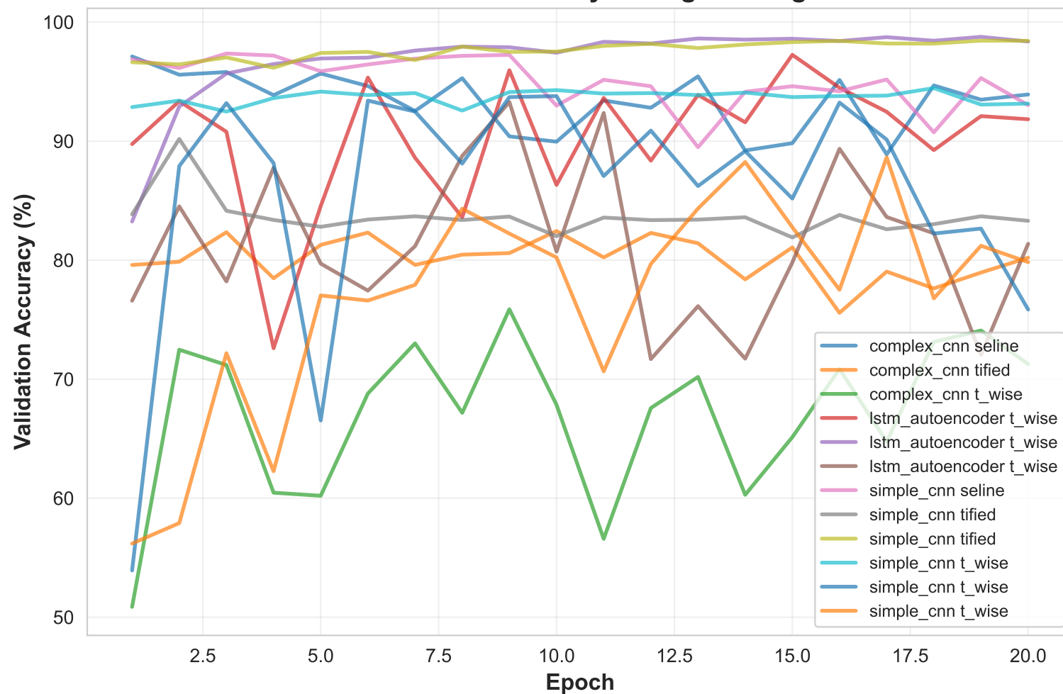
Validation Accuracy During Training
