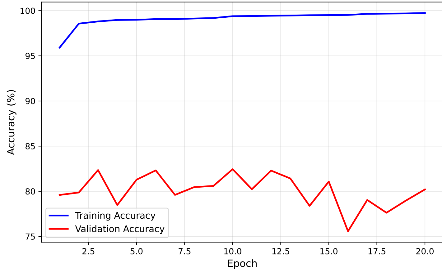
COMPLEX CNN - Training and Validation Accuracy
