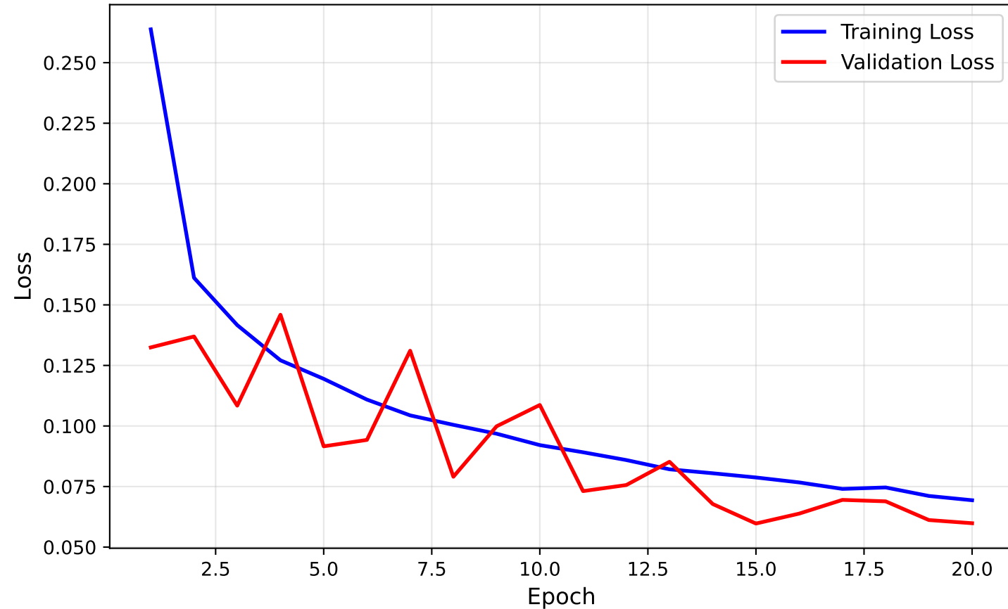
SIMPLE CNN - Training and Validation Loss
