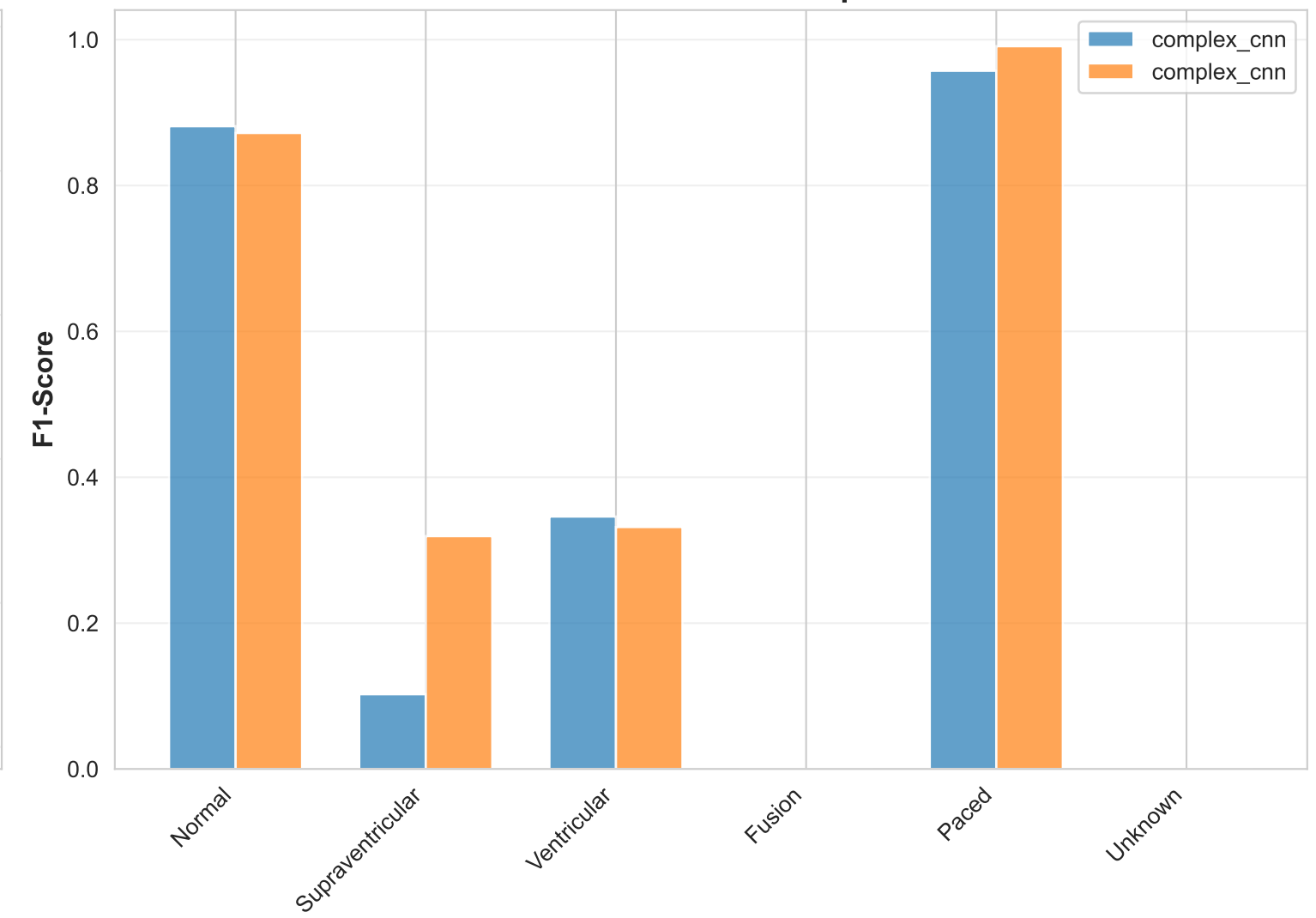
Per-Class F1-Score Comparison
