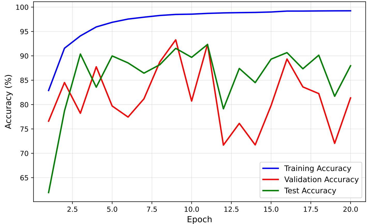
LSTM AUTOENCODER - Training/Val/Test Accuracy
