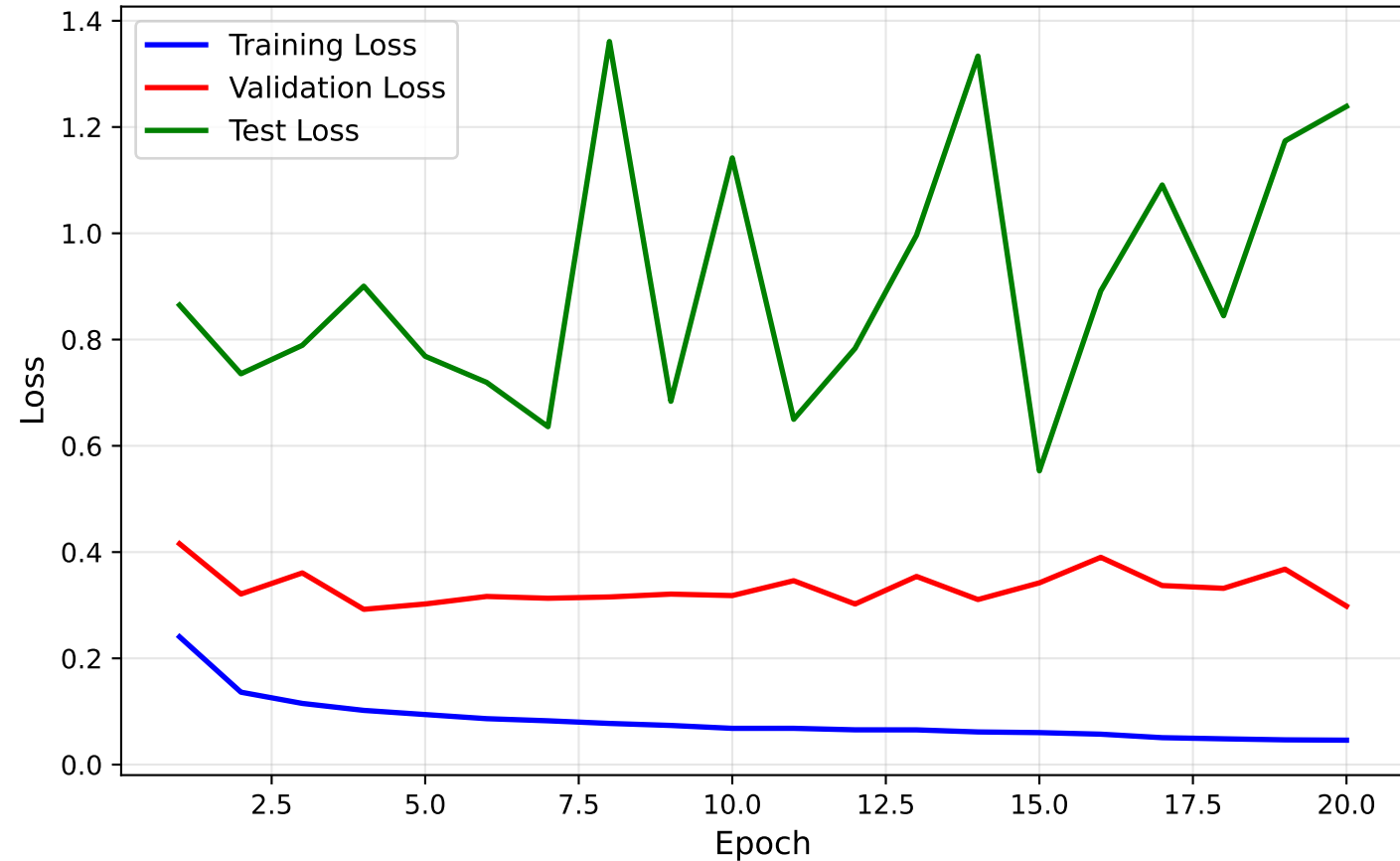
SIMPLE CNN - Training/Val/Test Loss
