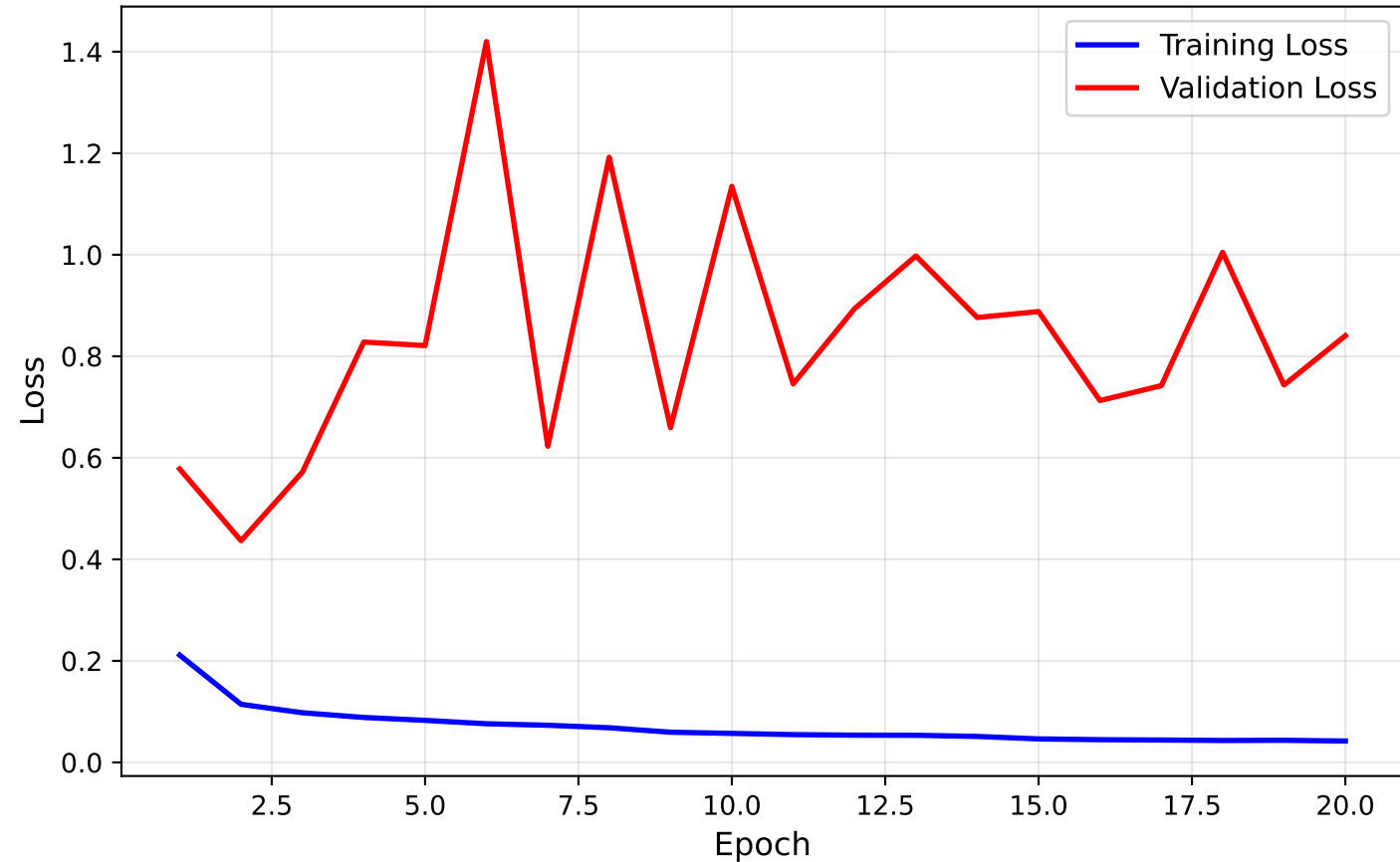
SIMPLE CNN - Training and Validation Loss
