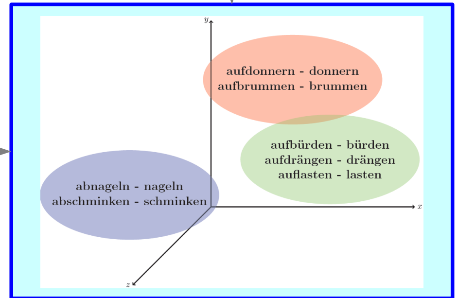
Distributional Analogy
