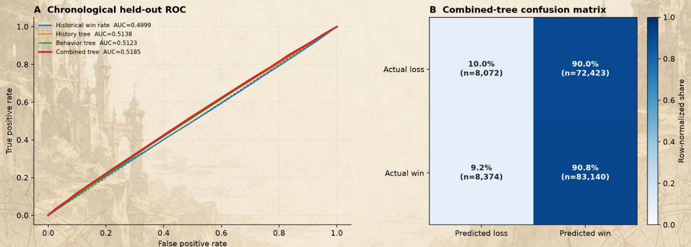
Figure 3. Chronological held-out predictive performance. The combined history + behavior tree improves ROC-AUC only slightly over the history-only model, while the normalized confusion matrix shows that the model identifies wins much more readily than losses.
