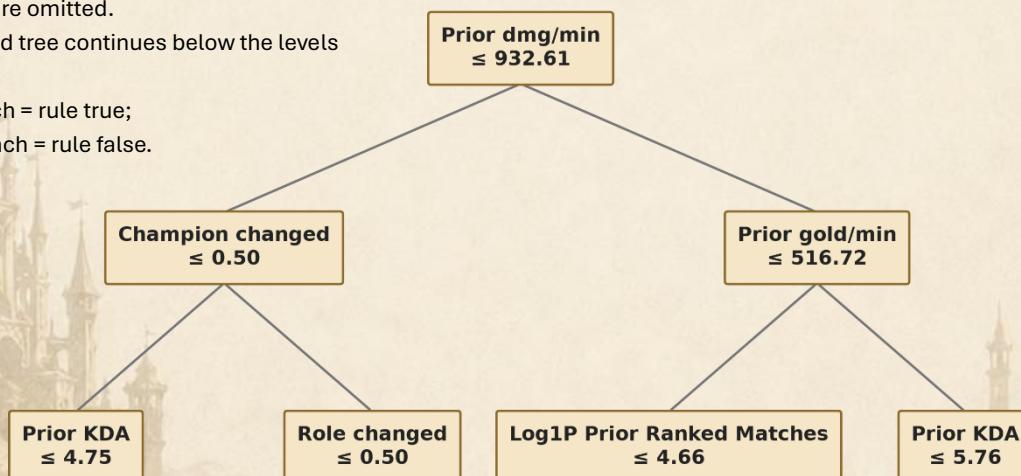
Figure 5. Top three levels of the combined entropy-based decision tree. The first splits are driven mainly by prior performance statistics, illustrating how the model separates observations before incorporating weaker behavioral features.
