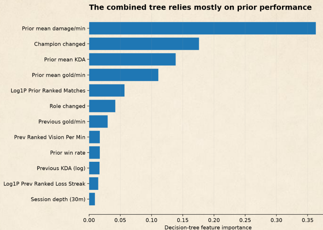
Figure 4. Feature importance of the combined entropy-based decision tree. Historical performance features account for most of the model's splitting decisions, while session and requeue-related variables contribute comparatively little.
