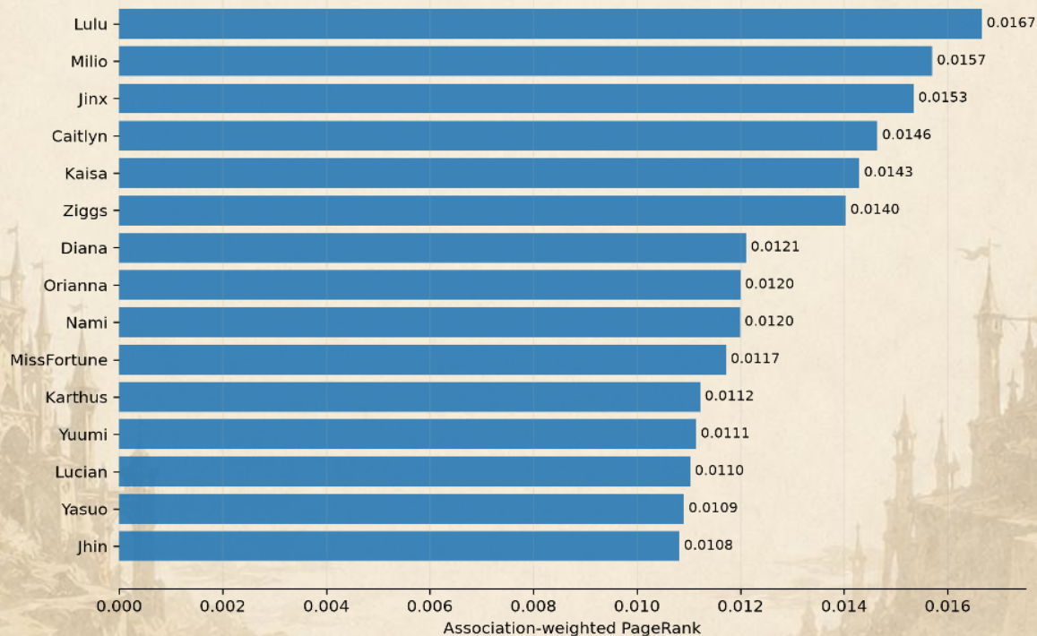
Figure 10. Association-weighted PageRank of the most structurally central champions.
