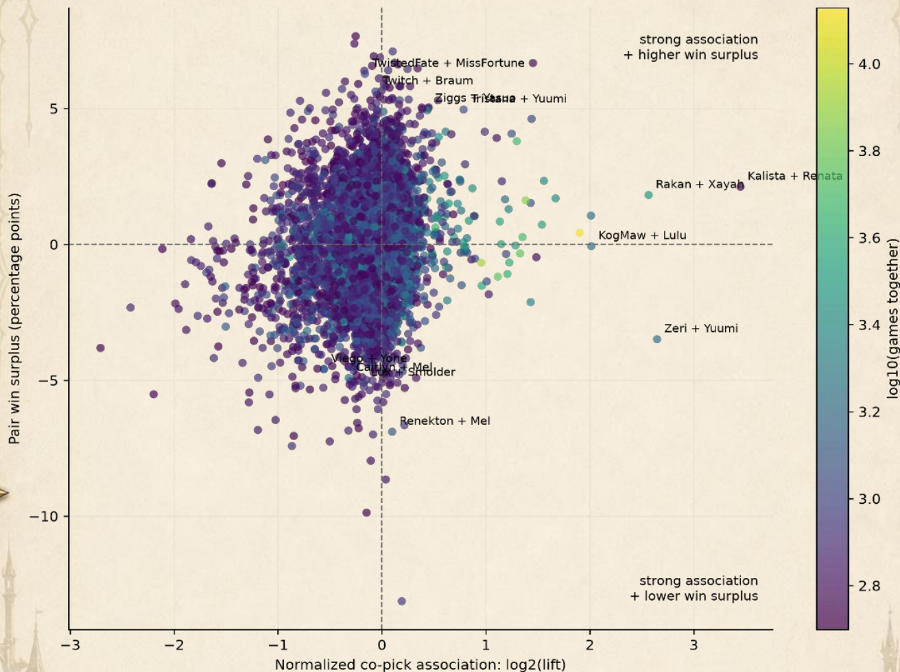
Figure 7. Champion co-selection strength versus pair win surplus. Strong association and strong performance are distinct properties.
