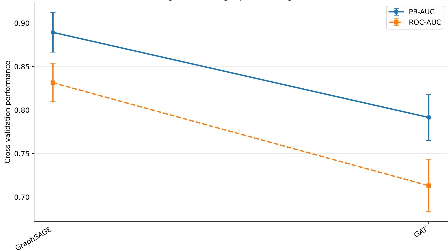
Progression of graph learning models
