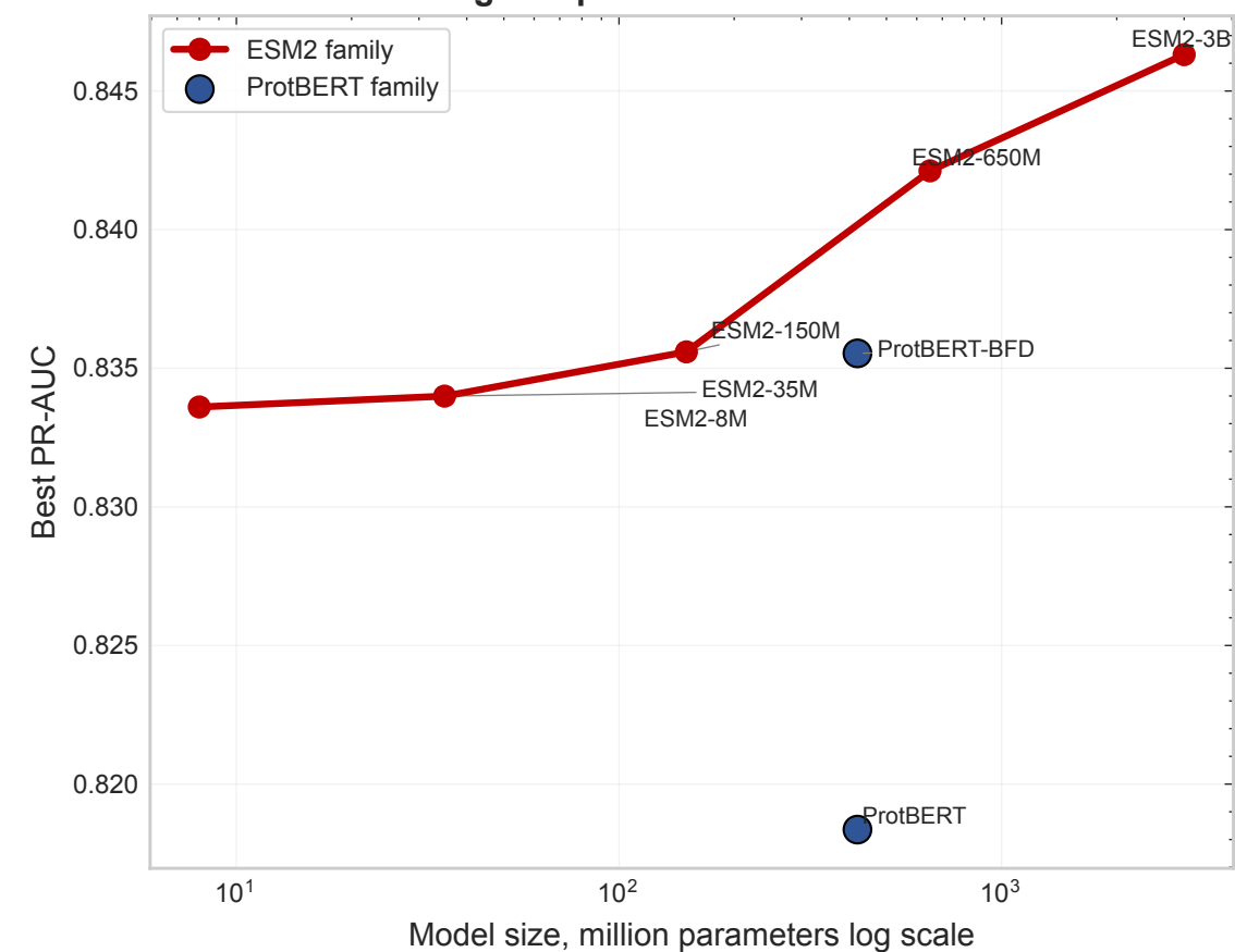
B. Parameter scaling and performance saturation
