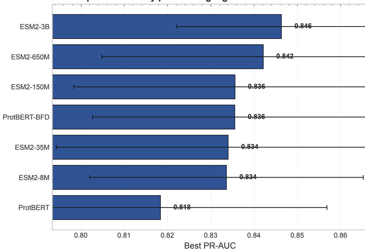
A. Best performance by protein language model
