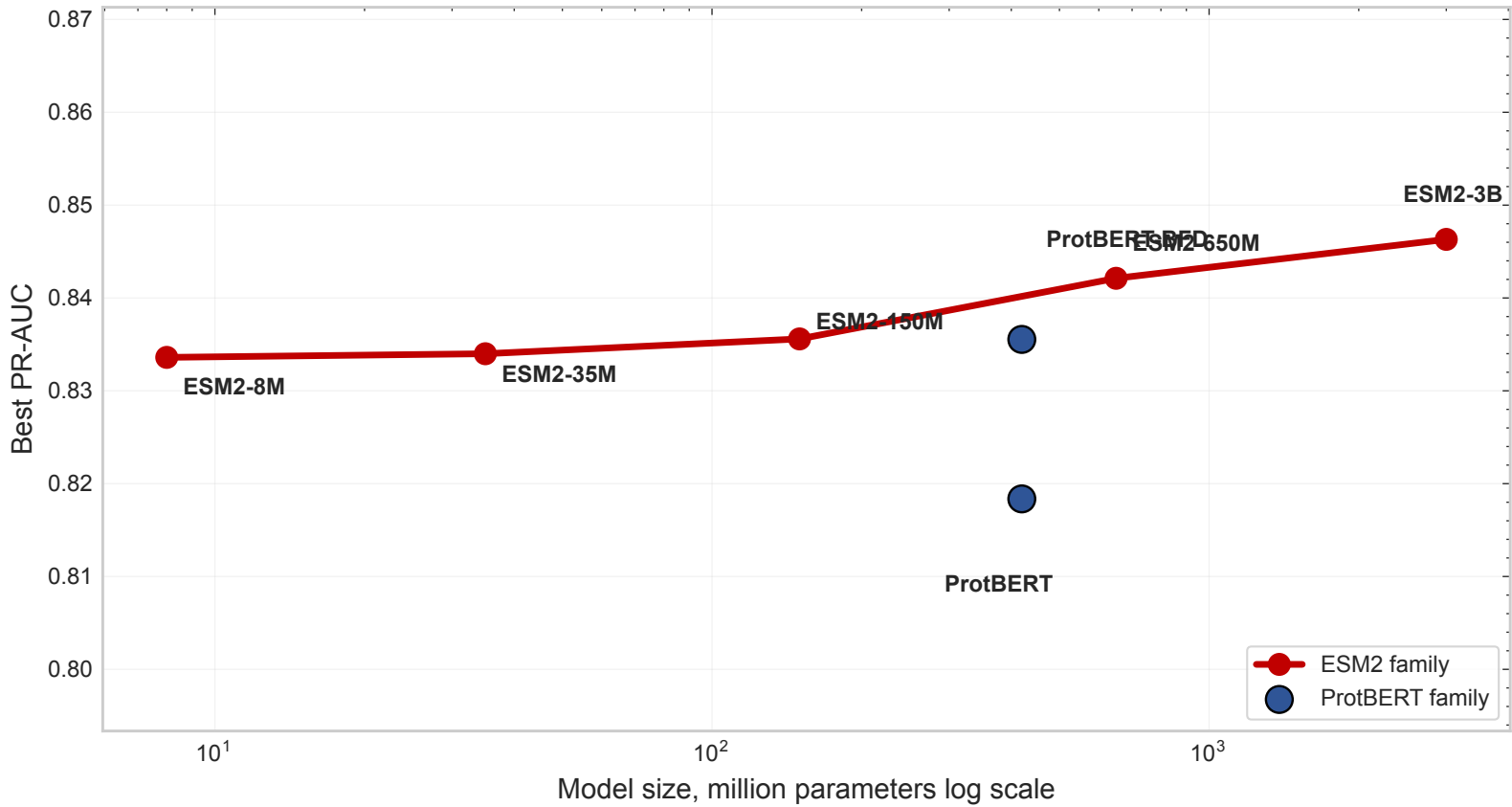
B. Parameter scaling and performance saturation
