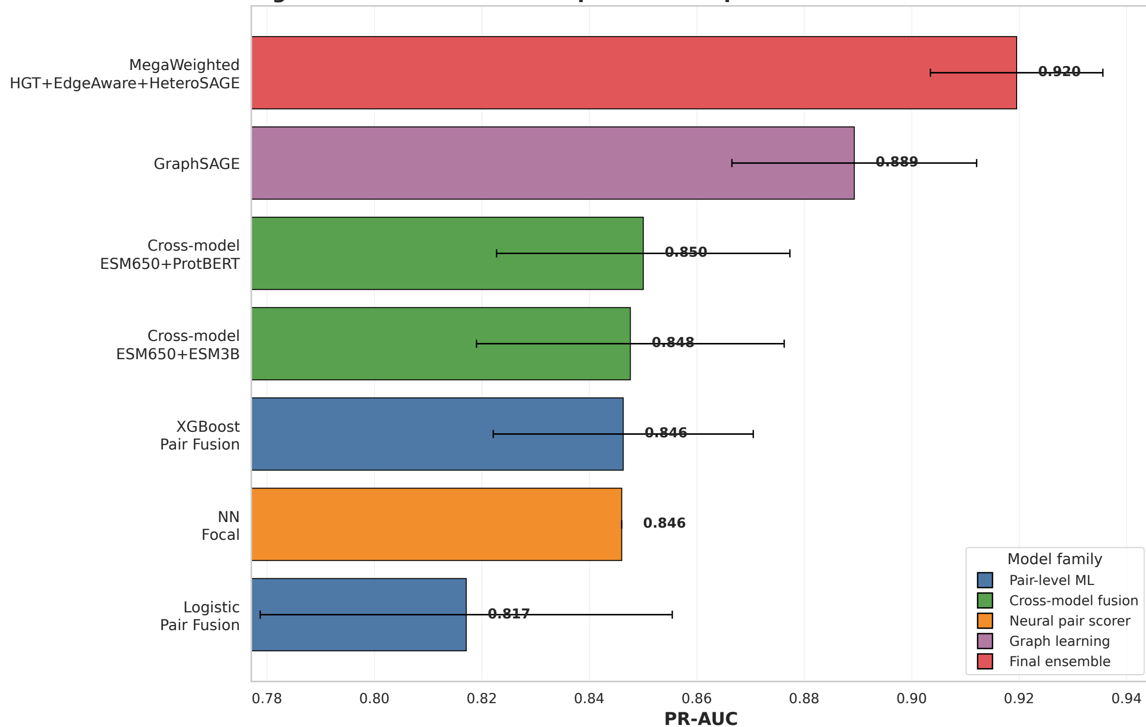
Figure 4A. Performance comparison of representative model families
