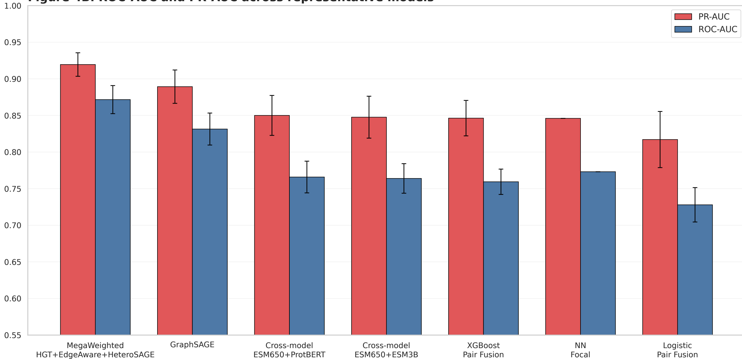
Figure 4B. ROC-AUC and PR-AUC across representative models
