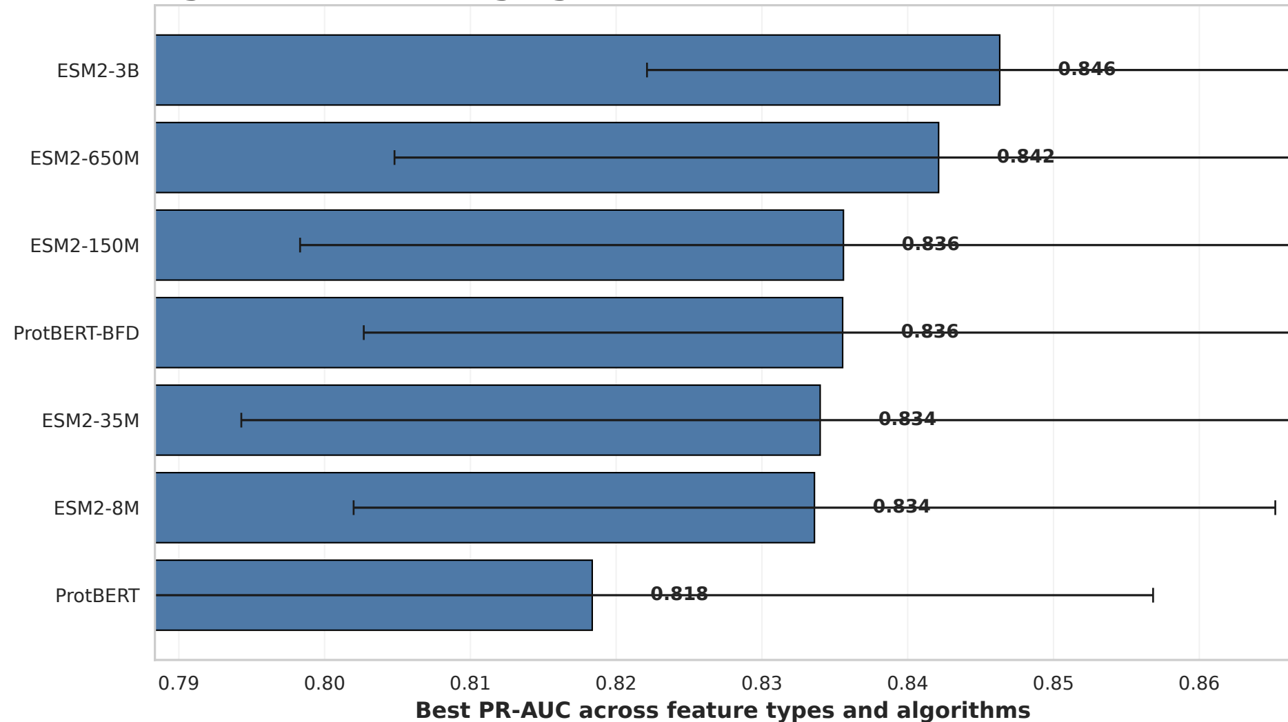
Figure 4E. Protein language model benchmark
