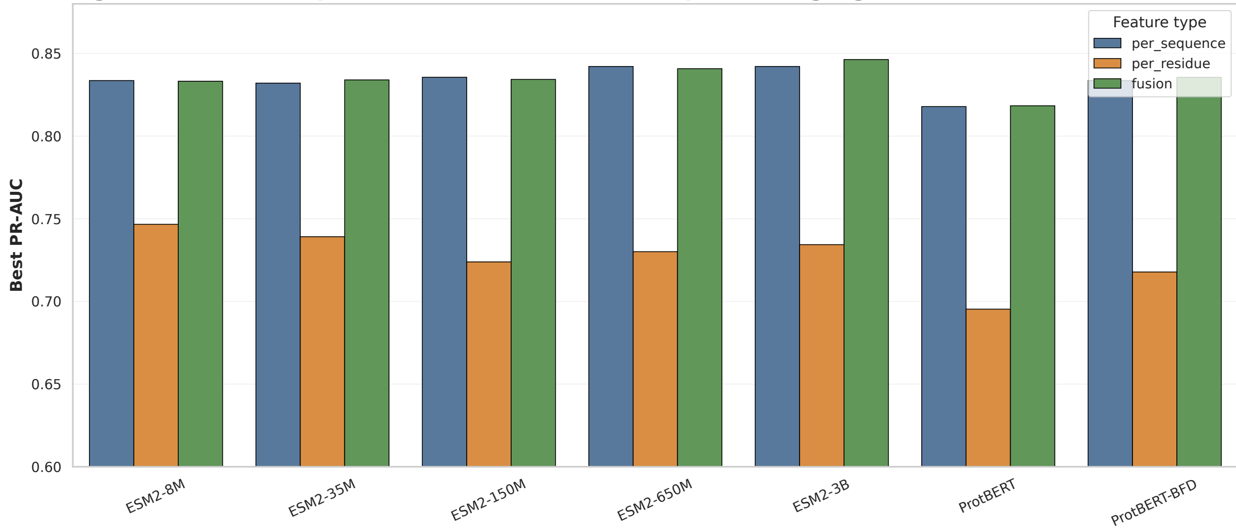
Figure 4G. Feature representation benchmark across protein language models
