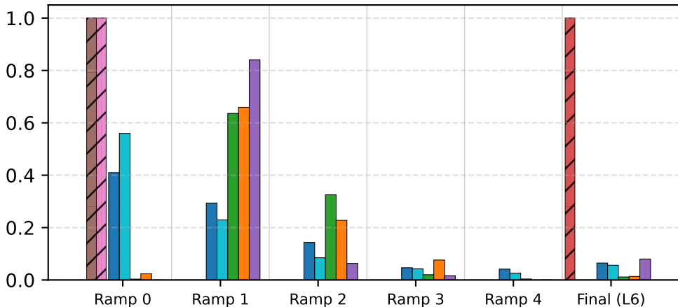
Fraction of docs exiting at layer
