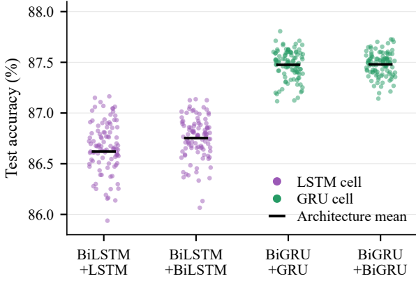
Fig. 1. Five-seed mean accuracy for each activation pair, grouped by architecture. Black horizontal markers show architecture means. Of the 400 configurations, one falls below the plotted range, which starts at 85.8%: Hardswish + LeakyReLU in BiLSTM+LSTM (mean 82.06%, SD 9.27 percentage points).
