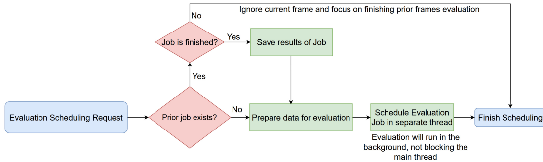
Figure 4.4: Flowchart of the background evaluation job scheduling
