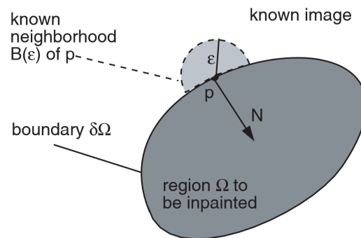
Figure 2.4: Taken from [Tel04]; Concept of the Fast-Marching Inpainting
