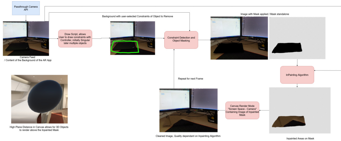
Figure 3.1: Flowchart visualization of the prototypes' workflow
