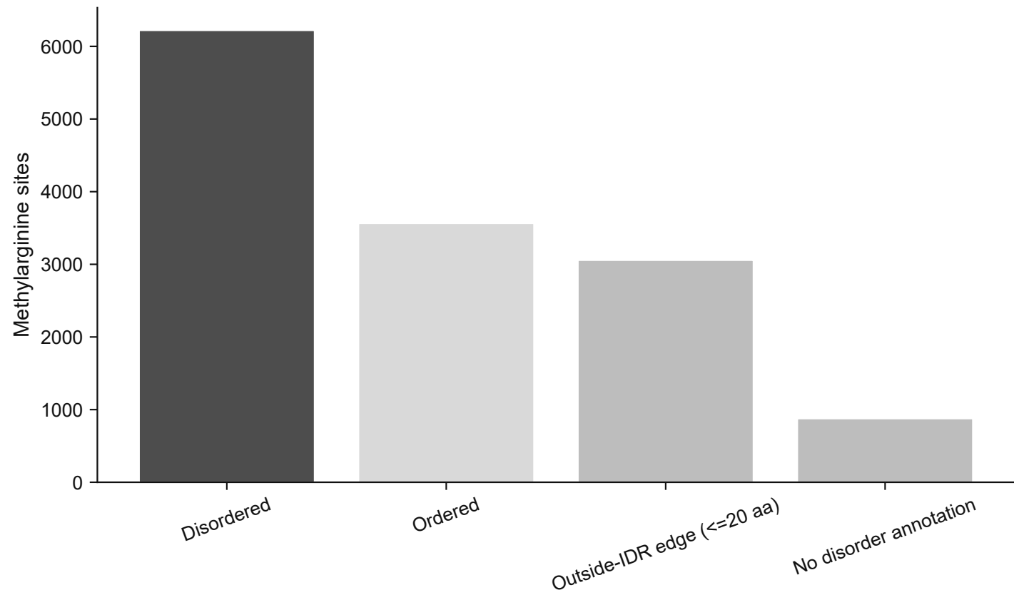
Methylarginine disorder-context distribution
