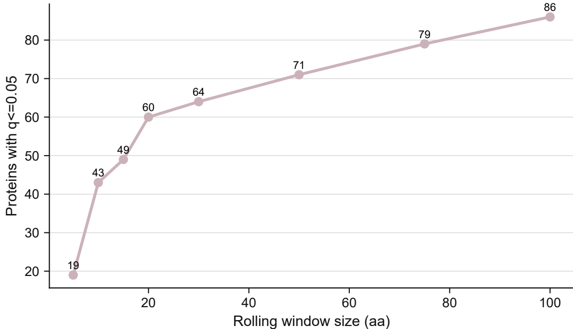
Significant methylarginine clustering across window sizes
