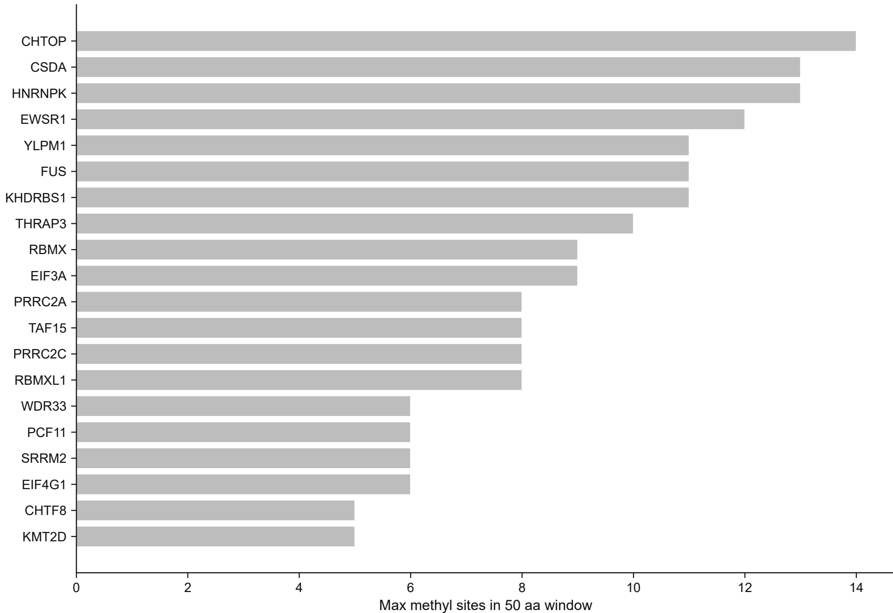
Top proteins by local methylarginine density
