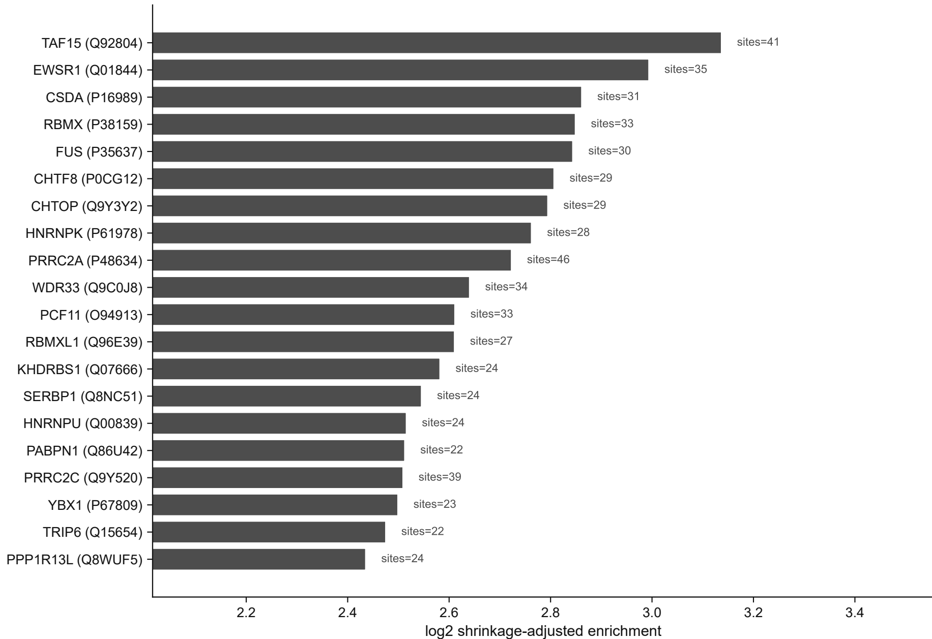
Top proteins by shrinkage-adjusted methylarginine enrichment
