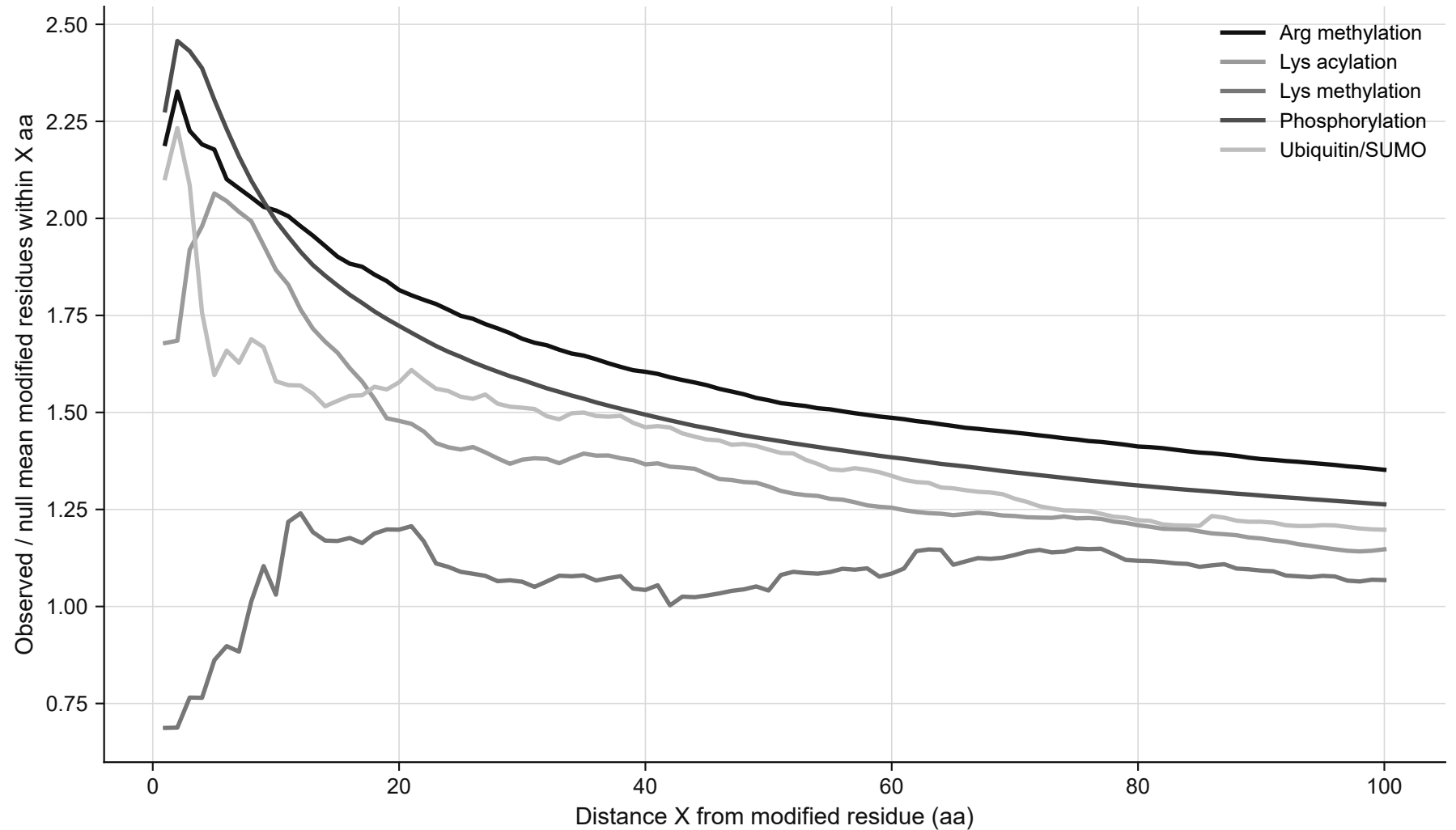
Cross-PTM local density enrichment vs null
