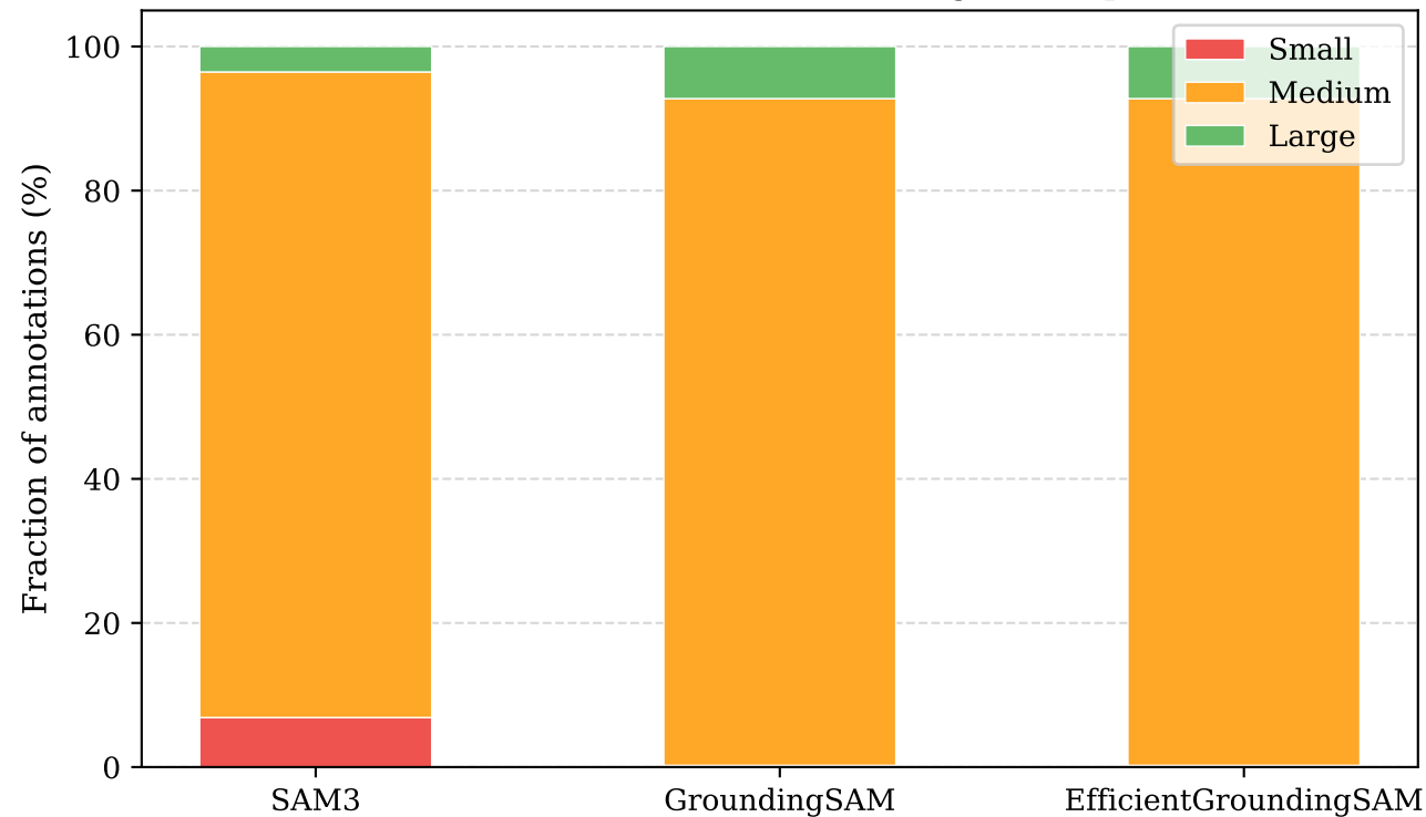
COCO Size Class Distribution (small \leq 32^2 , medium \leq 96^2 , large > 96^2 px)
