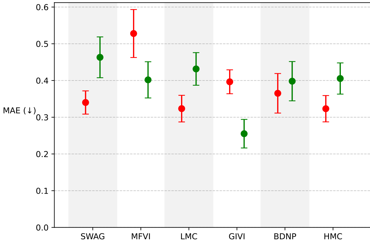
heaviside
