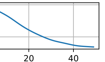
autocorrelation
