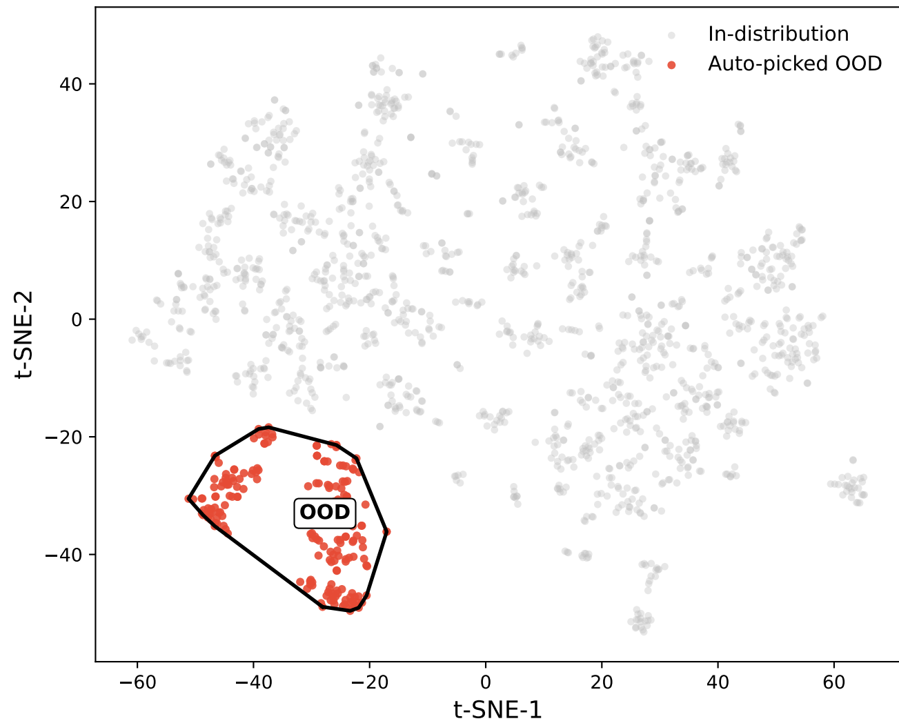
t-SNE projection with auto-selected OOD cluster
