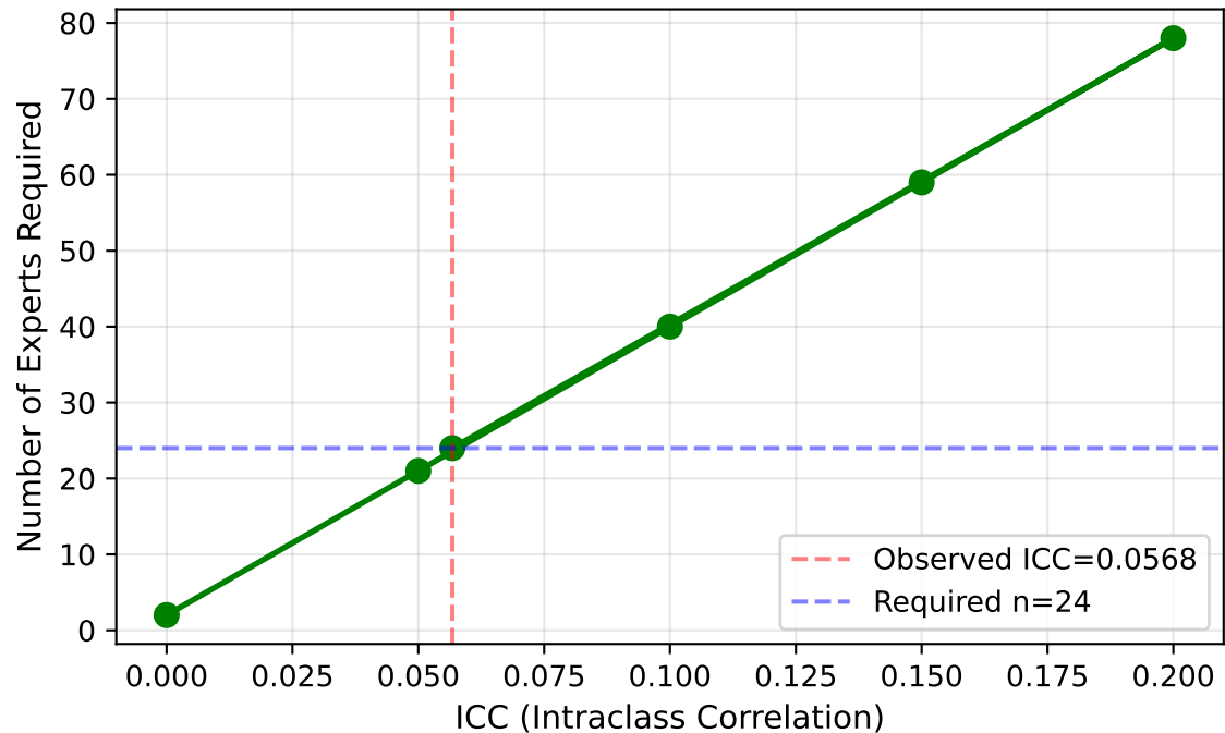
Required Experts for \pm 5\% Margin of Error
