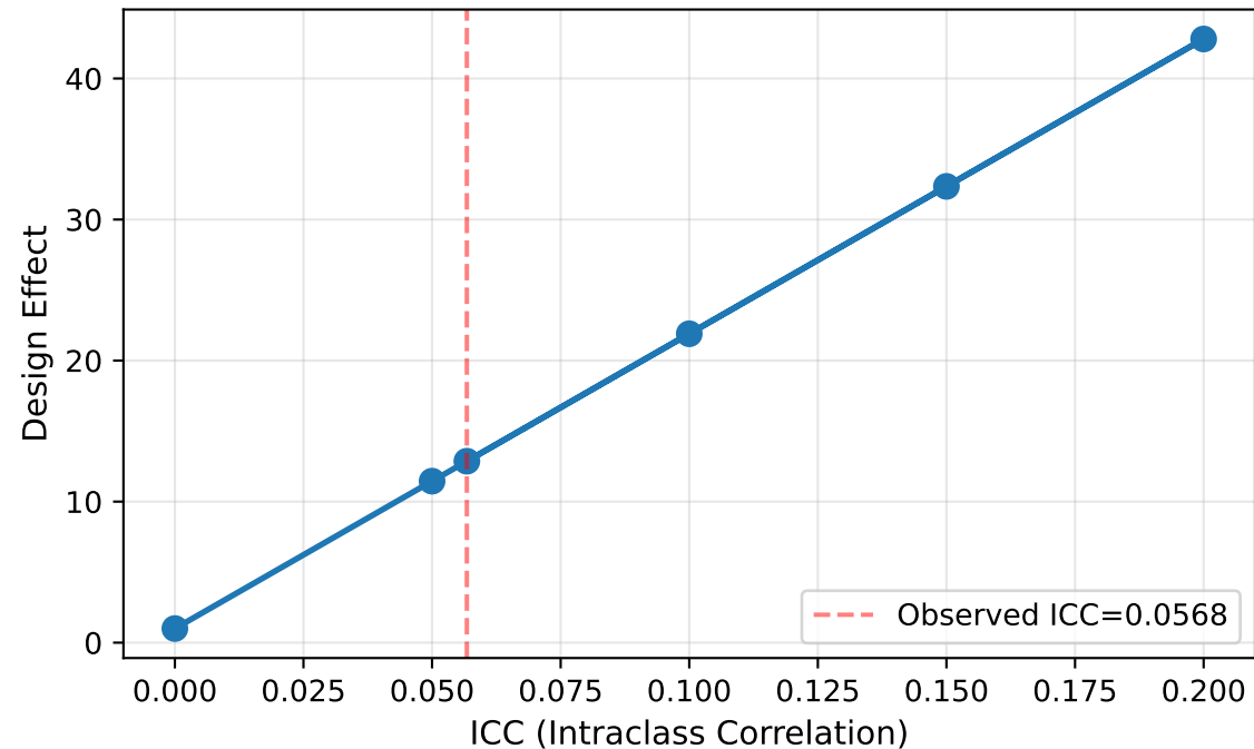
Impact of ICC on Design Effect
