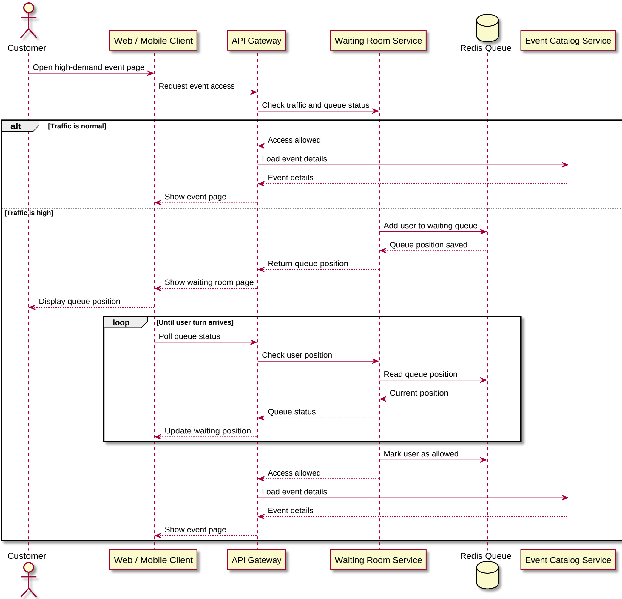
Sequence Diagram 02 - Virtual Waiting Room Flow
