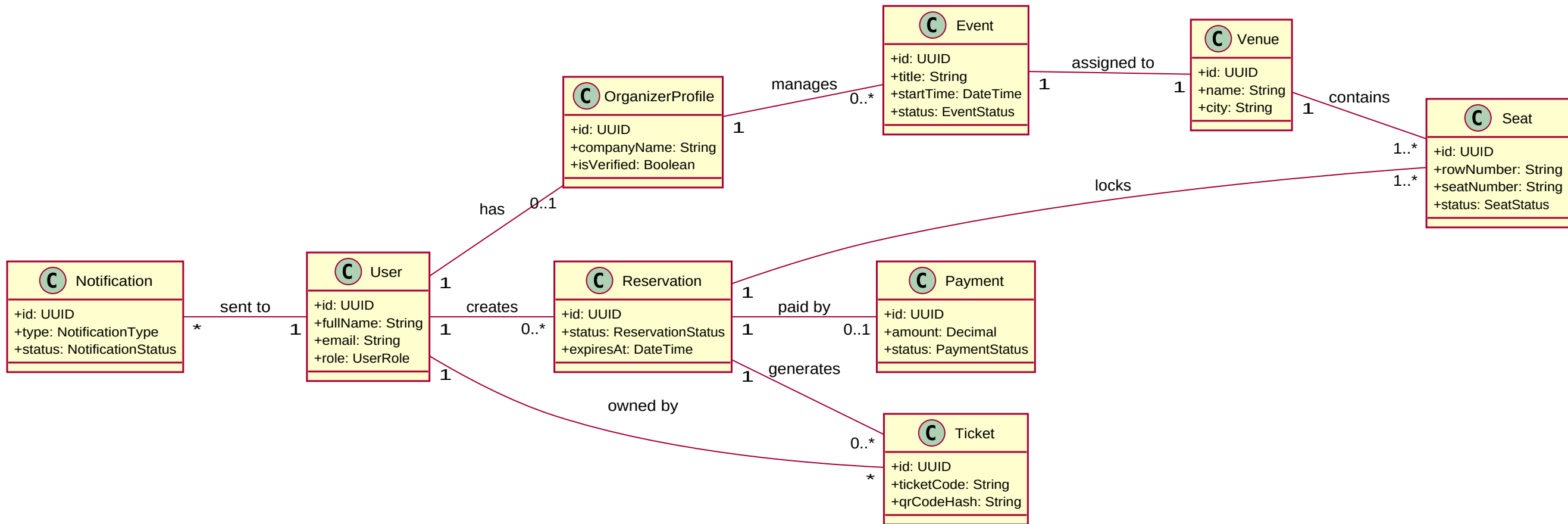
Class Diagram 01 - Core Domain Overview
