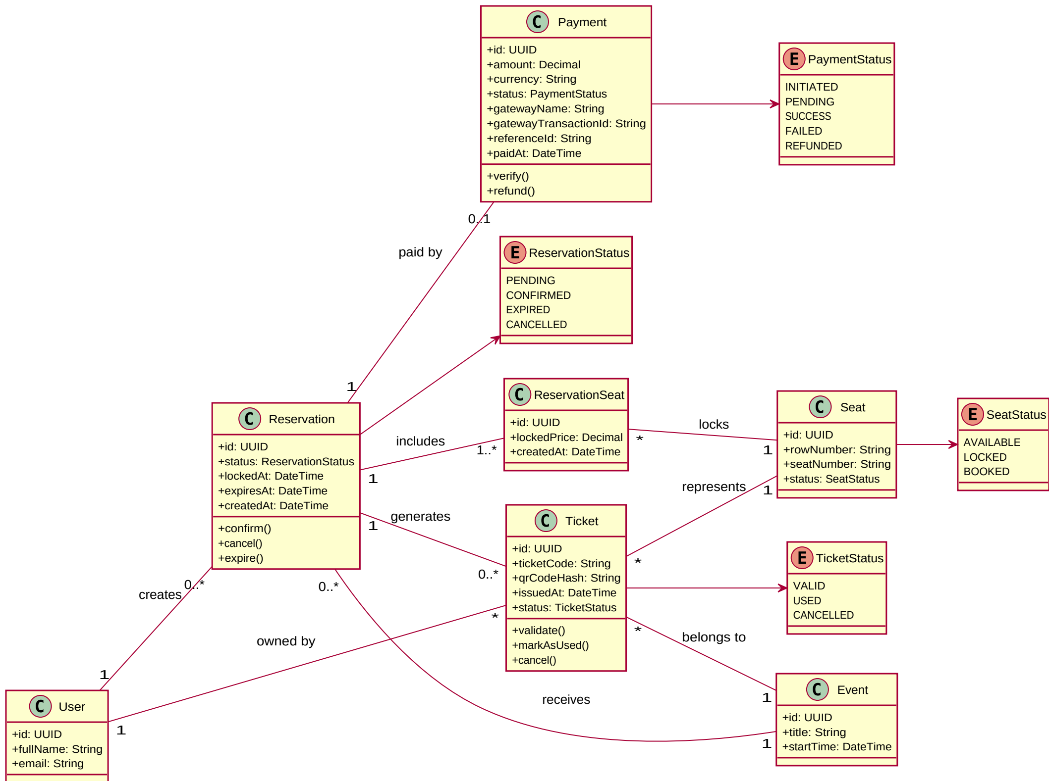
Class Diagram 04 - Reservation, Payment and Ticket Model
