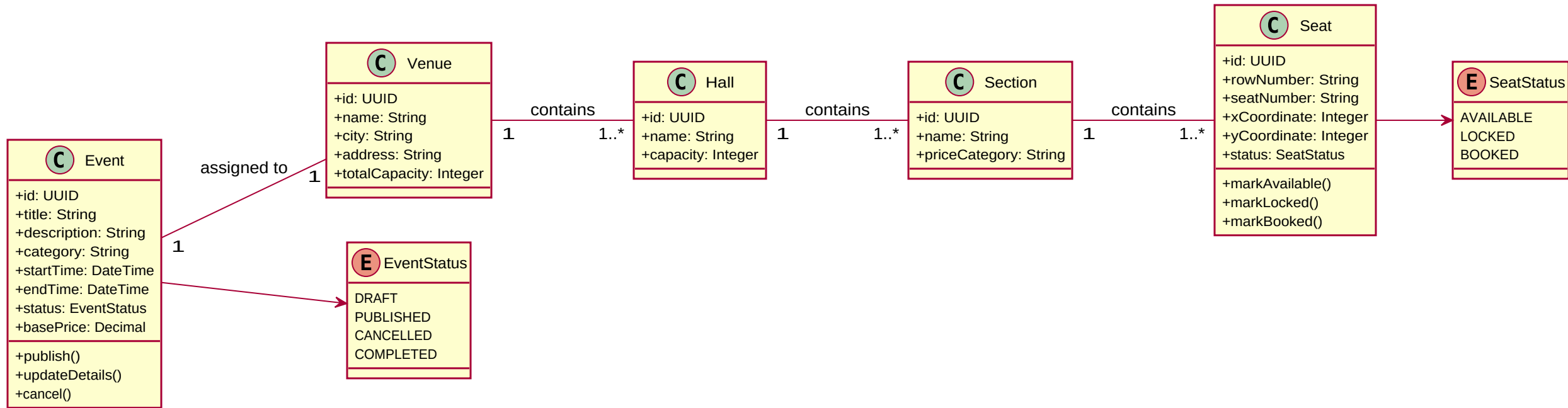
Class Diagram 03 - Event, Venue and Seat Model
