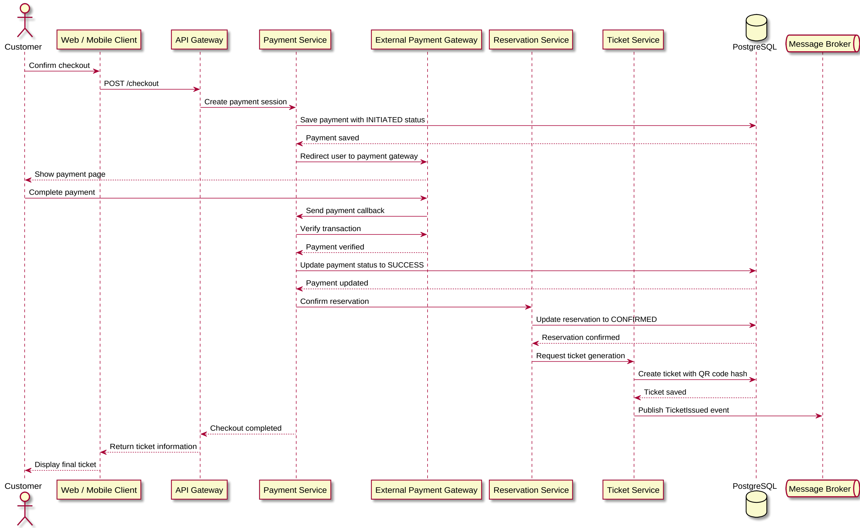
Sequence Diagram 04 - Payment Success and Ticket Issuance
