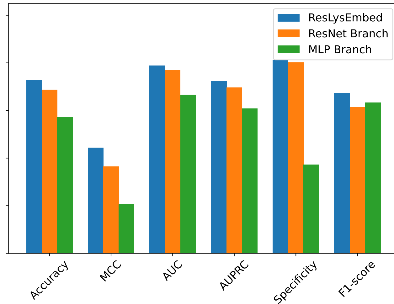
dbPTM Test Dataset
