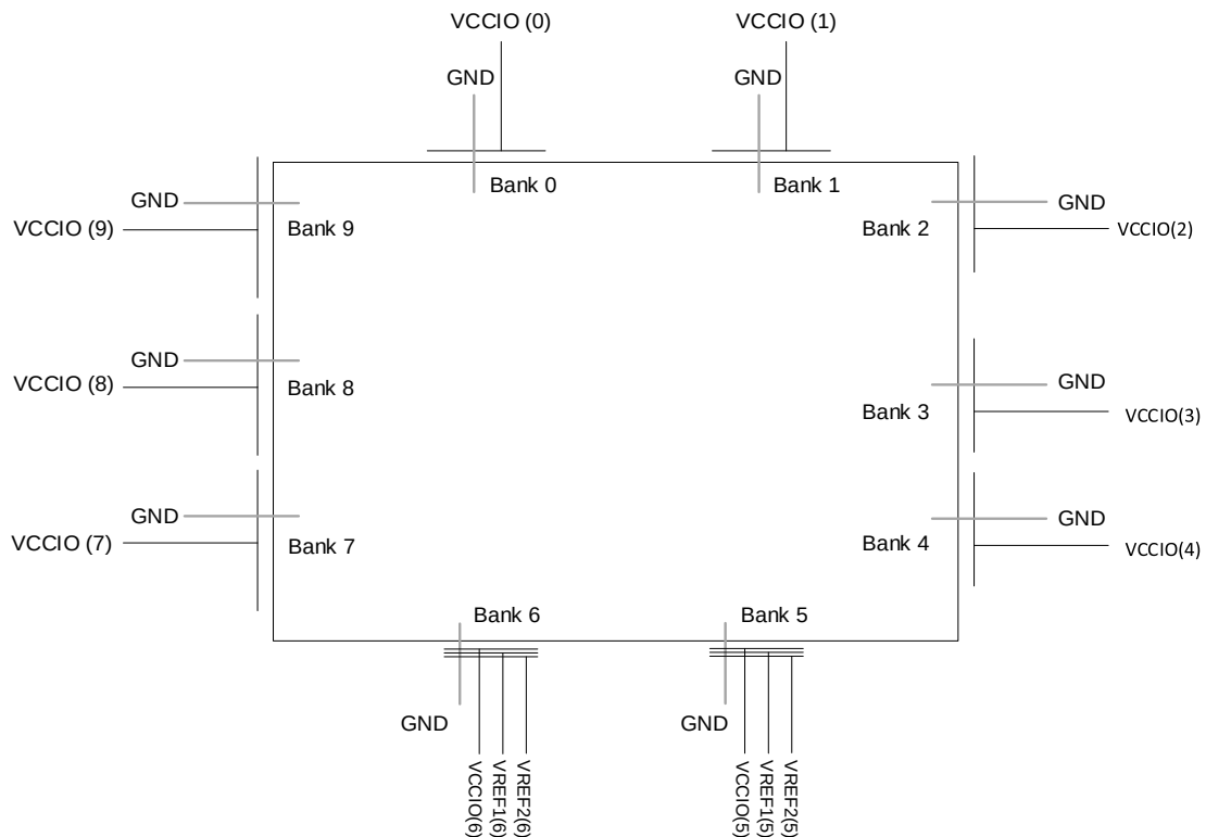
Figure 3.2. LFMXO5-25/LFMXO5-15D sys/O Banking
