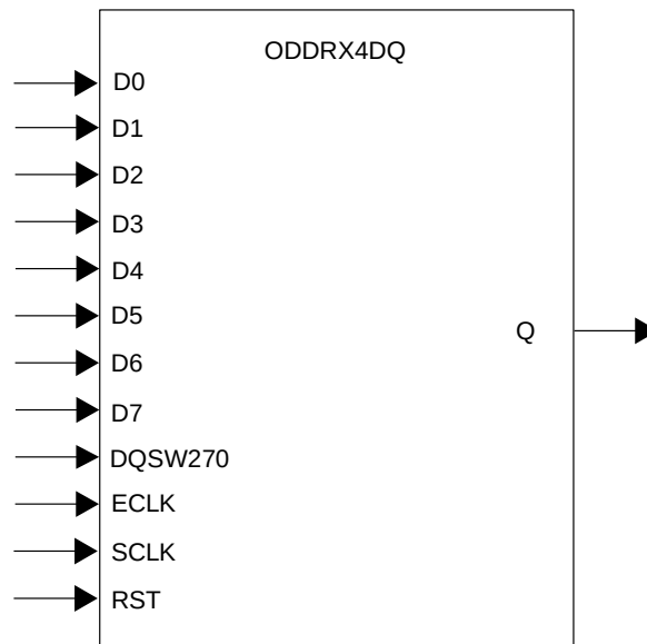
Figure 8.18. ODDRX4DQ Primitive
