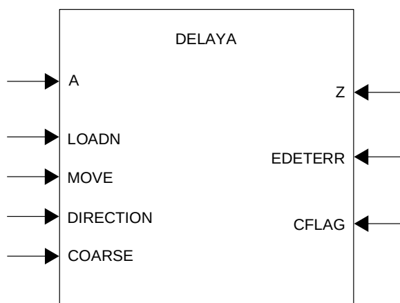
Figure 8.1. DELAYA Primitive
