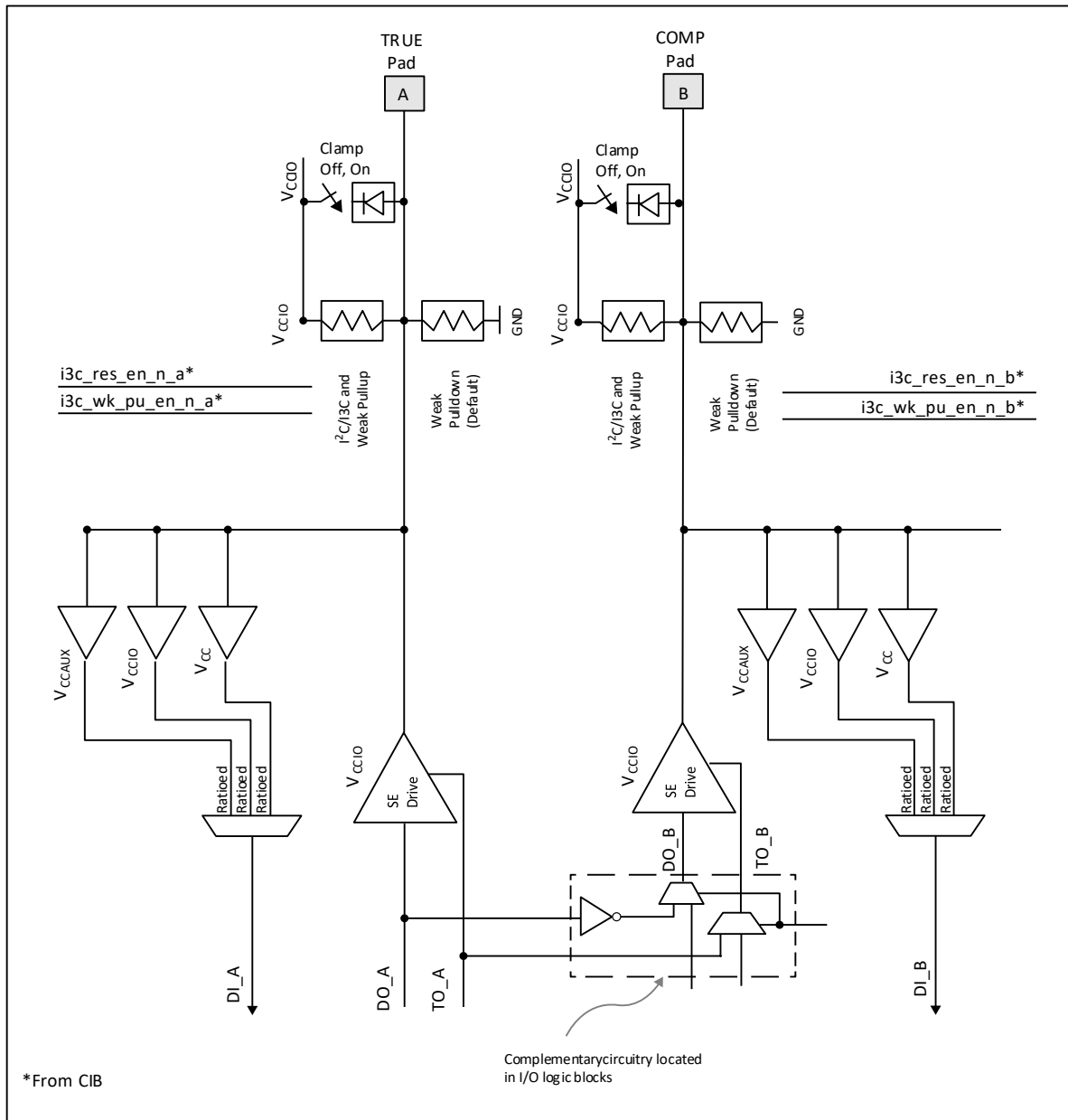
Figure 3.7. Wide Range sys/O Buffer for Top, Left/Right Side
