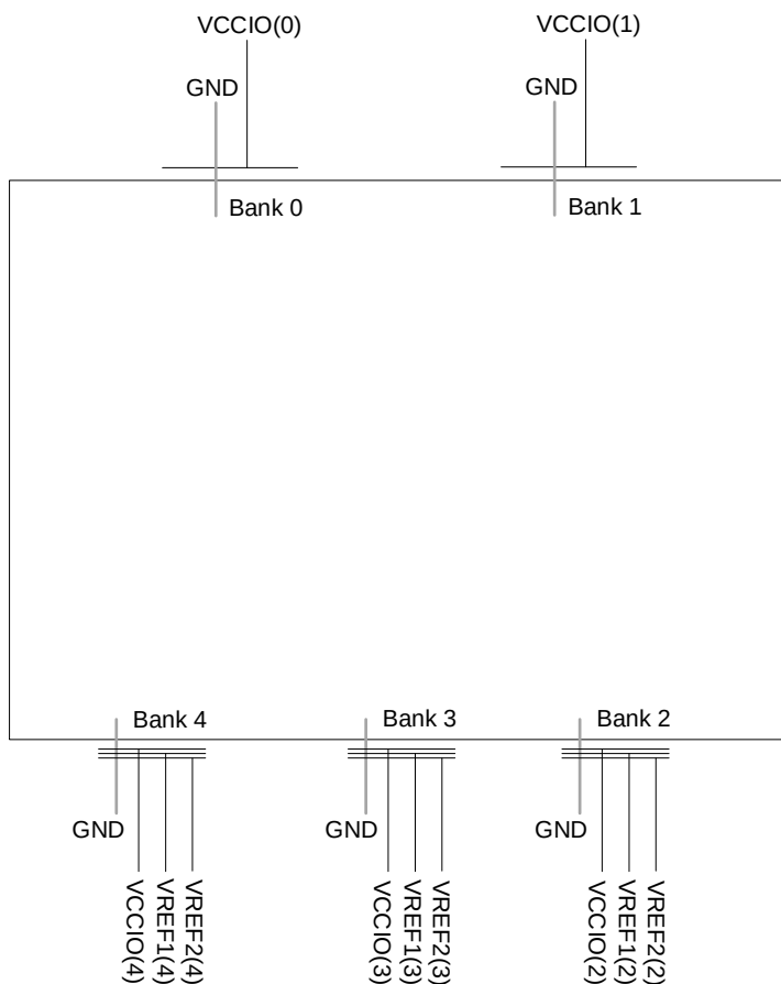
Figure 3.5. CrossLinkU-NX sysI/O Banking
