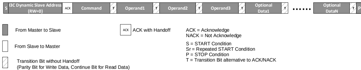
Figure 6.40. Typical I3C Write without 7'h7E
