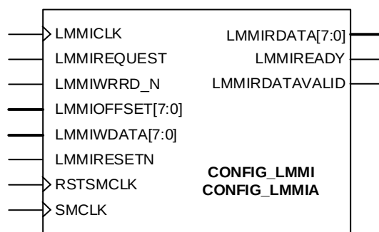
Figure D.1. CONFIG_LMMI(A) Primitive Pin Diagram
