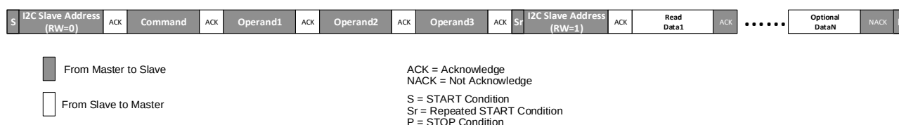
Figure 6.36. Typical I 2 C Read
