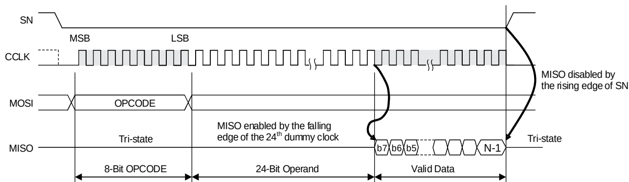
Figure 6.25. Class A Command Waveforms
