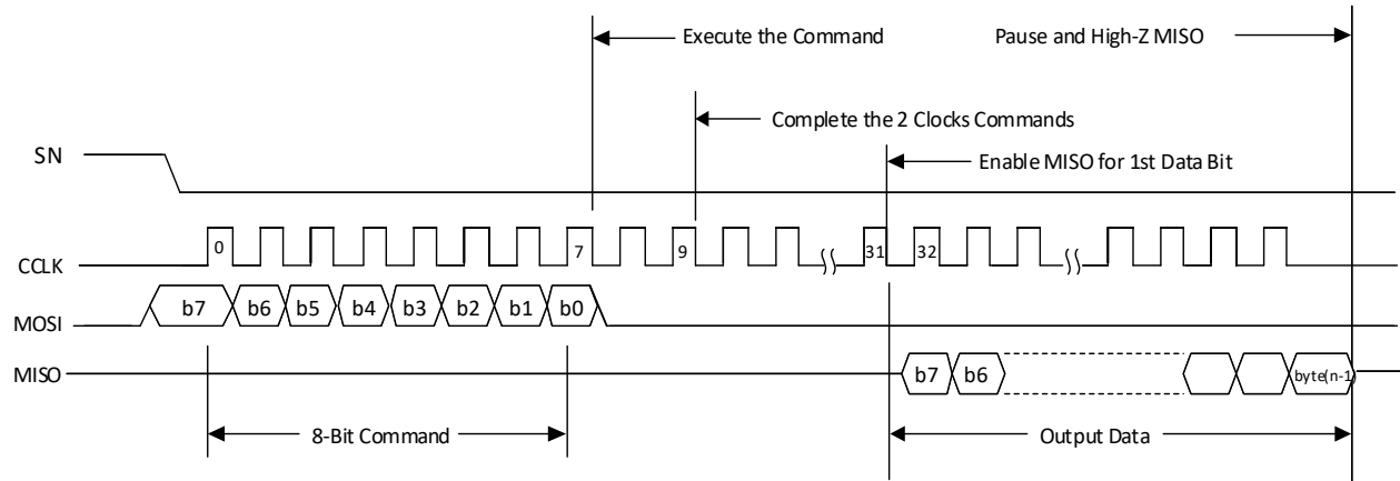
Figure 6.22. Slave SPI Read Waveforms
