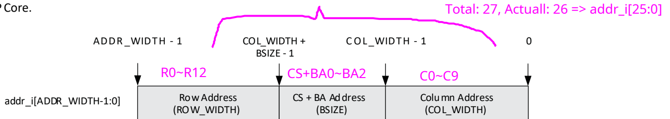
Figure 2.7. Local-to-Memory Address Mapping for Memory Access
