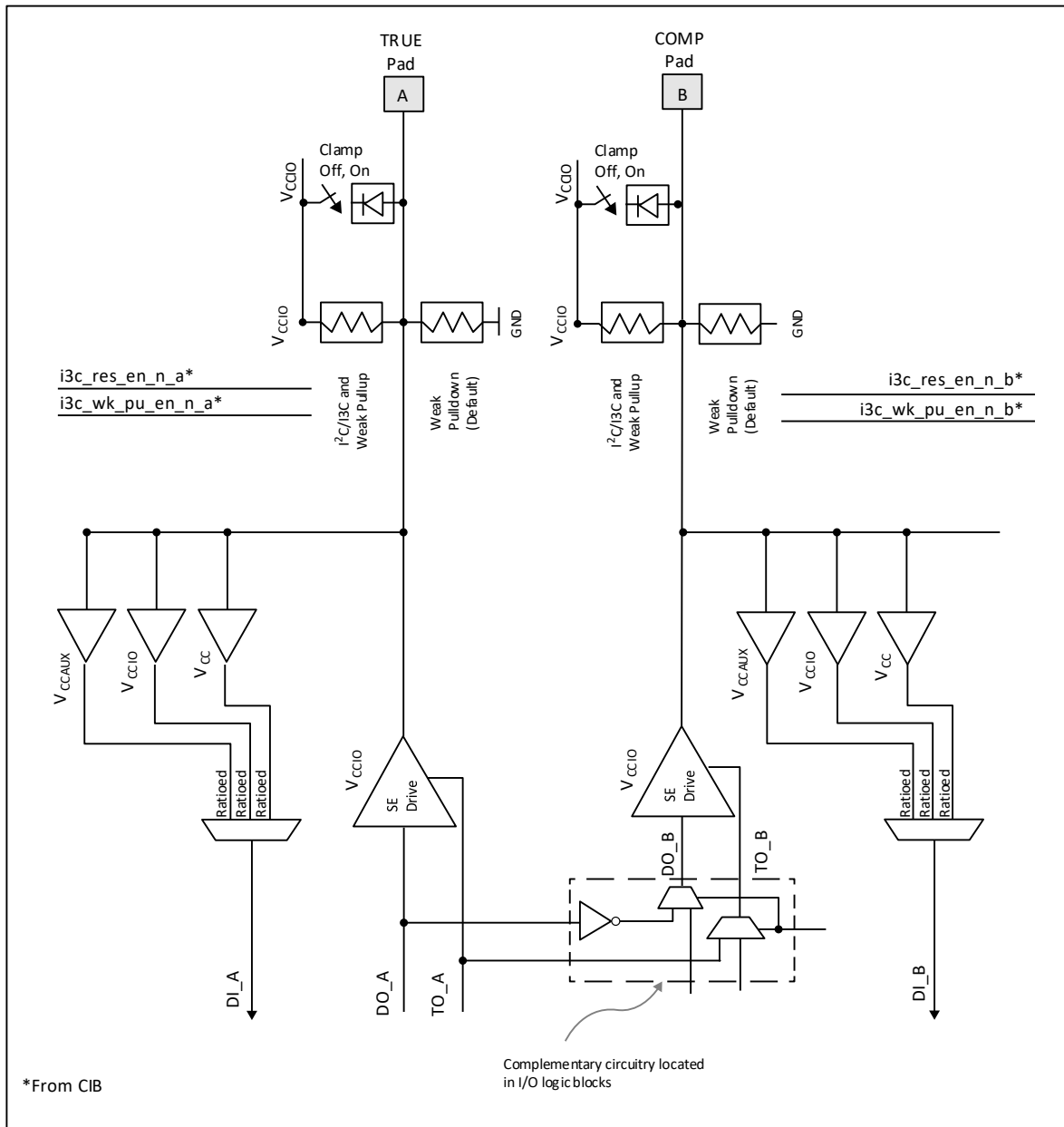
Figure 3.7. Wide Range sysI/O Buffer for Top, Left, or Right Side
