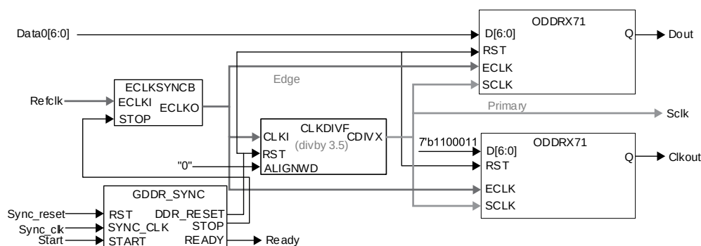
Figure 5.28. GDDR71_TX.ECLK Interface
