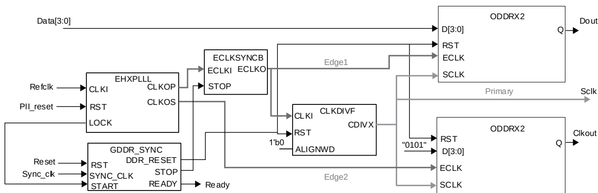
Figure 5.23. GDDR2_TX.ECLK.Centered Interface
