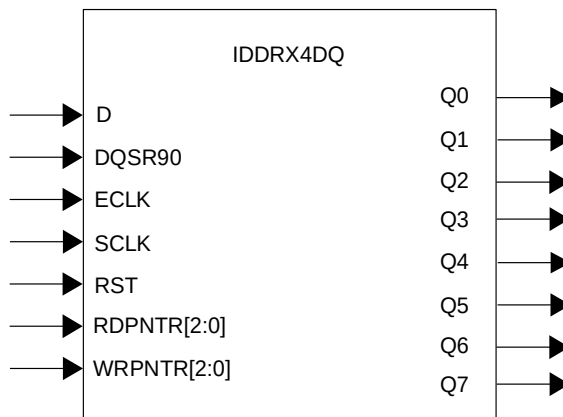
Figure 8.16. IDDRX4DQ Primitive
