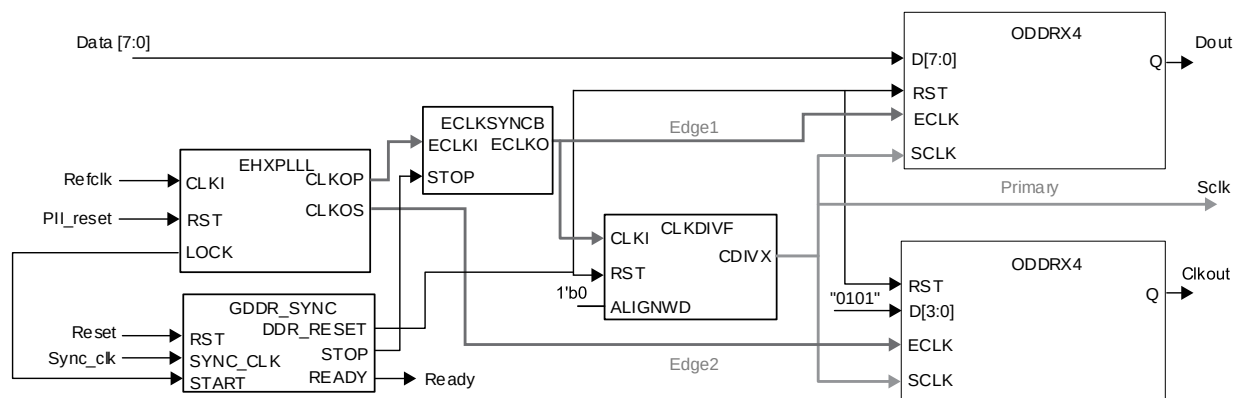
Figure 5.25. GDDR4_TX.ECLK.Centered Interface
