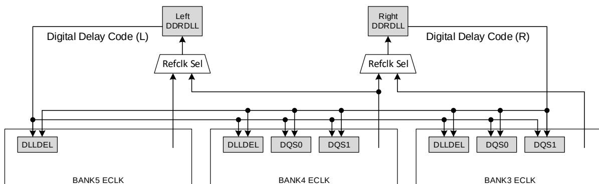
Figure 2.12. DDRDLL Architecture
