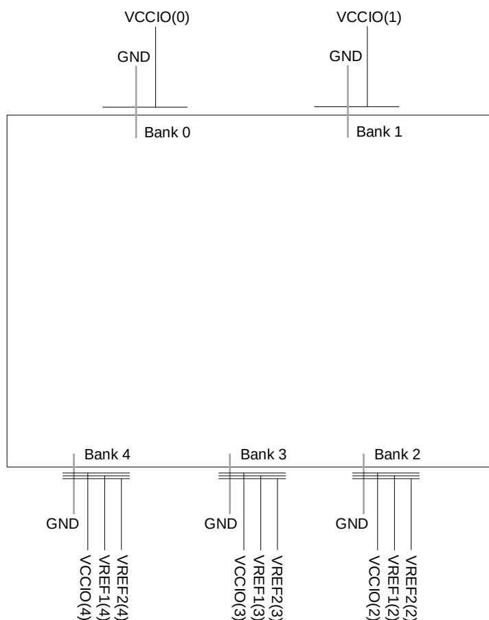
Figure 3.5. CrossLinkU-NX sysl/O Banking
