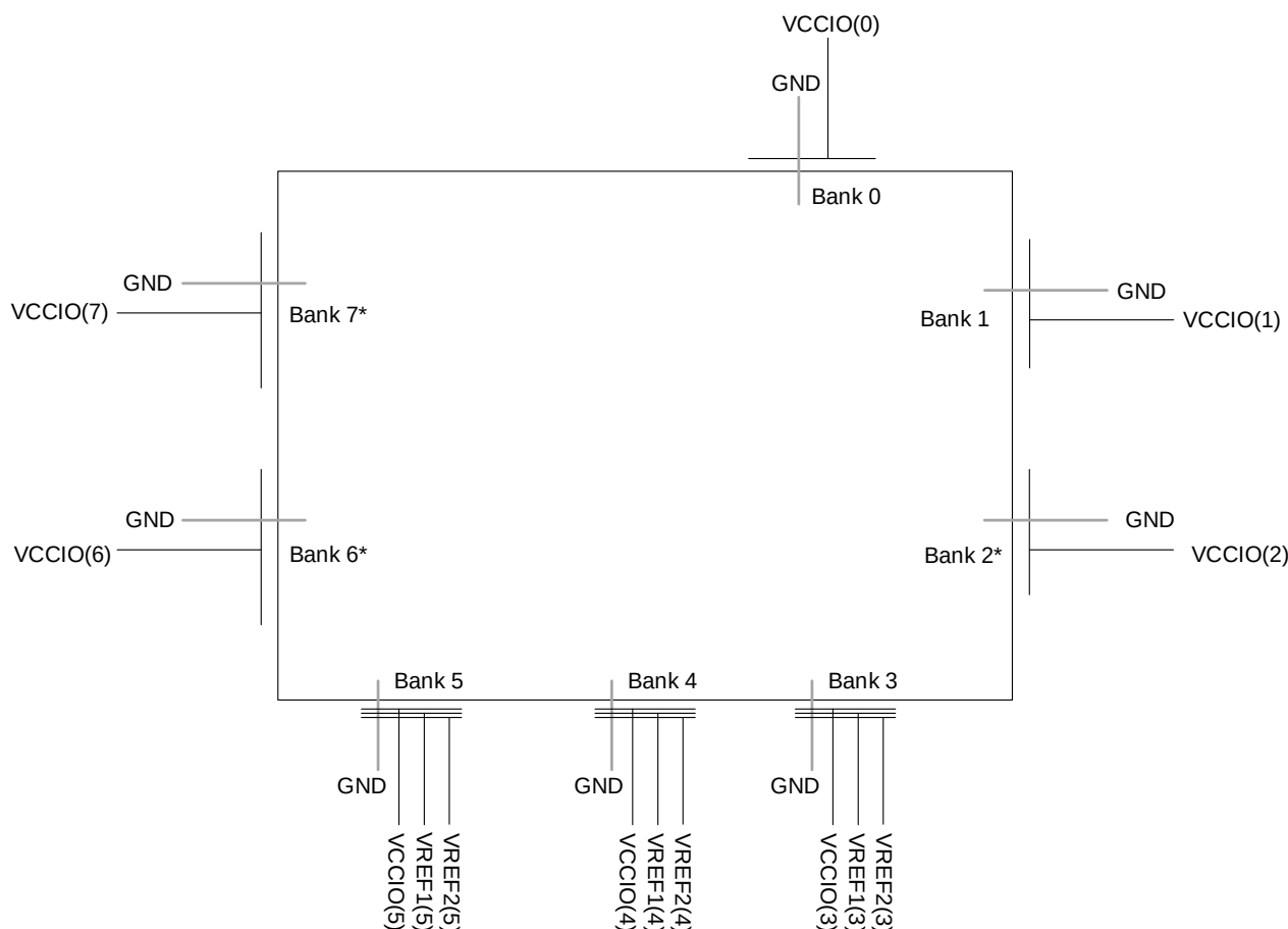
Figure 3.1. CrossLink-NX, Certus-NX, CertusPro-NX sysI/O Banking
