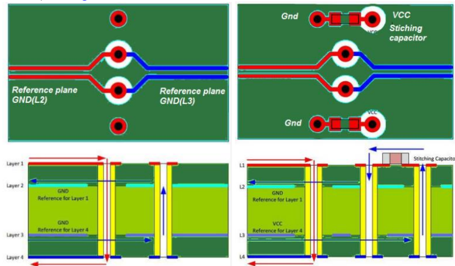
Figure 15.1. Recommended Layout
