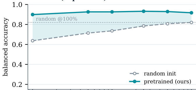
ISRUC (sleep)
