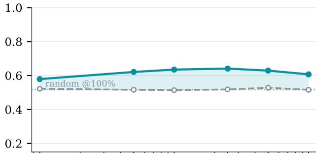
HMC (sleep)
