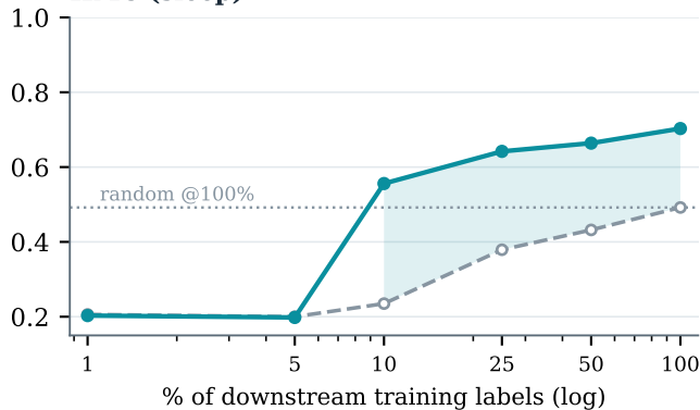
HMC (sleep)
