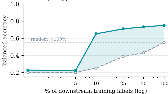
ISRUC (sleep)
